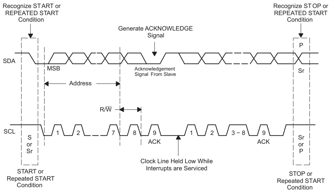
Figure 15. Bus Protocol
