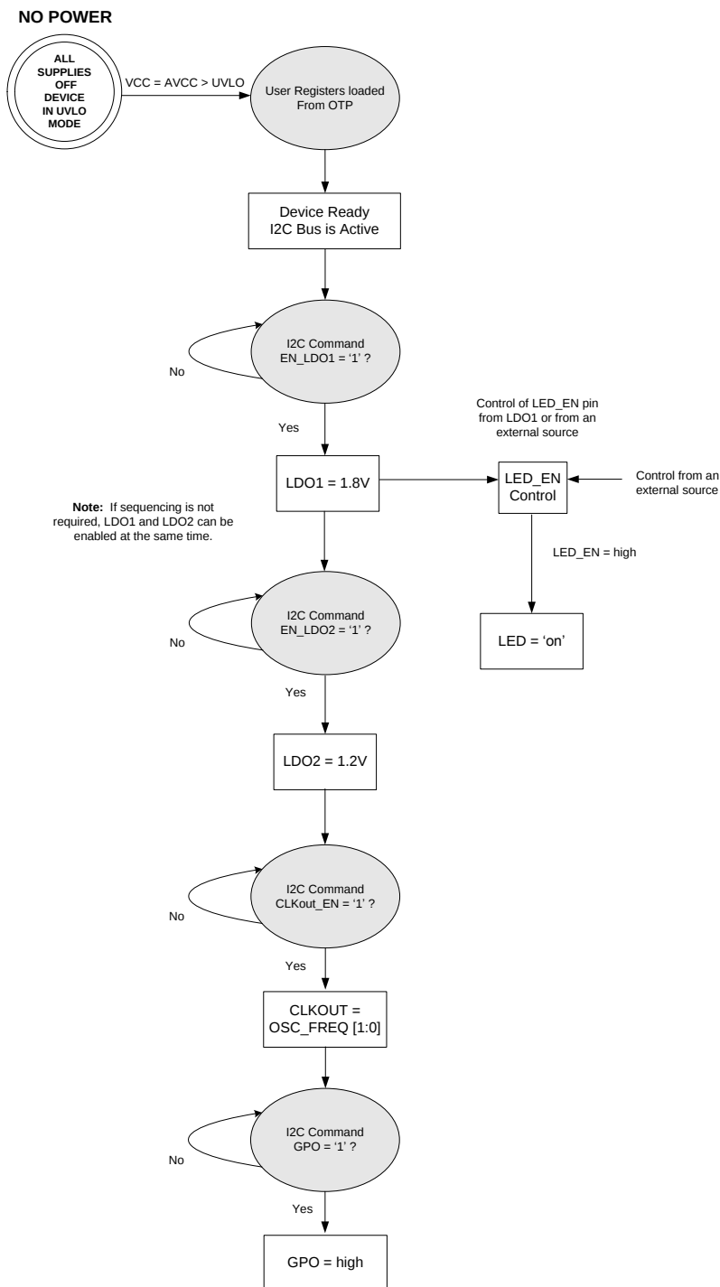
Figure 6. State Diagram
