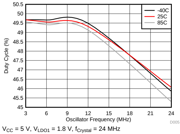
Figure 37. Duty Cycle
