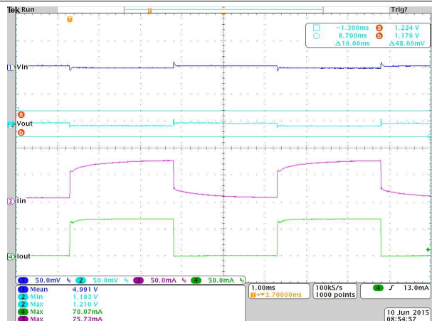
Figure 32. Line Transient Response LDO2
