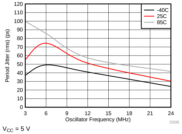
Figure 38. Period Jitter
