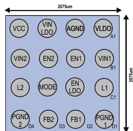
TPS657052 YZH Package 16-Pin DSBGA Top View
