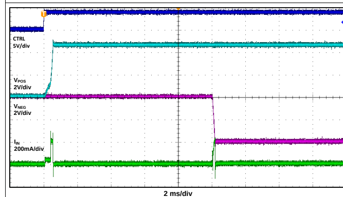
Figure 11. Start-Up Waveforms
