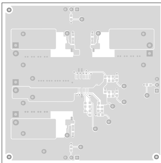
Figure 14. Top Layer
