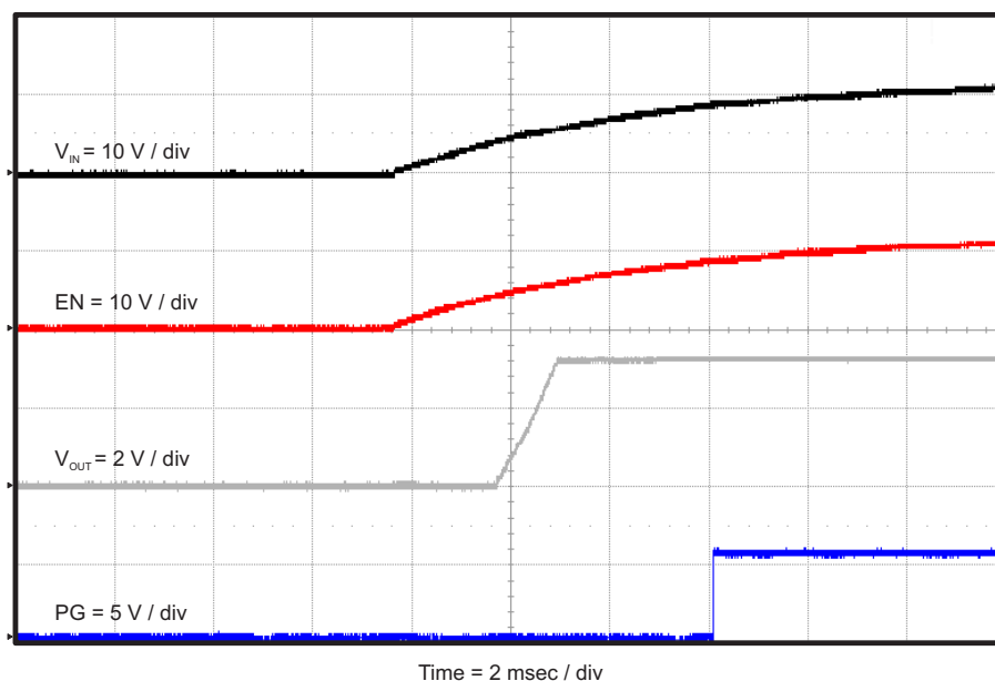
Figure 11. TPS65580EVM-575 CH1 Start-Up Relative to V_{IN}
