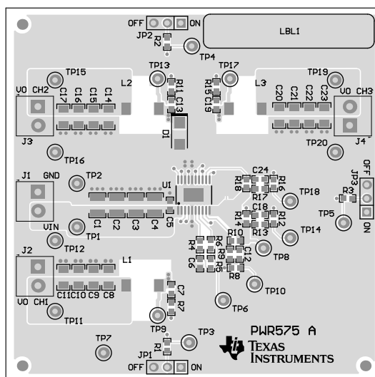
Figure 13. Top Assembly
