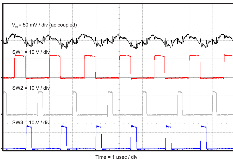
Figure 10. TPS65580EVM-575 Input Voltage Ripple
