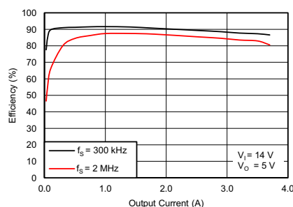
Buck Efficiency Versus Output Current
