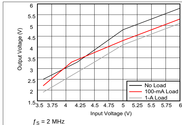
Figure 1. Buck-Regulator Output Voltage
