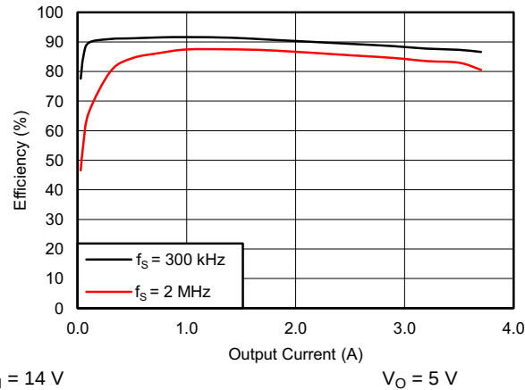
Figure 22. Buck Efficiency Versus Output Current
