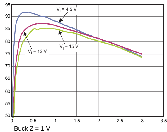
Figure 4. Efficiency
