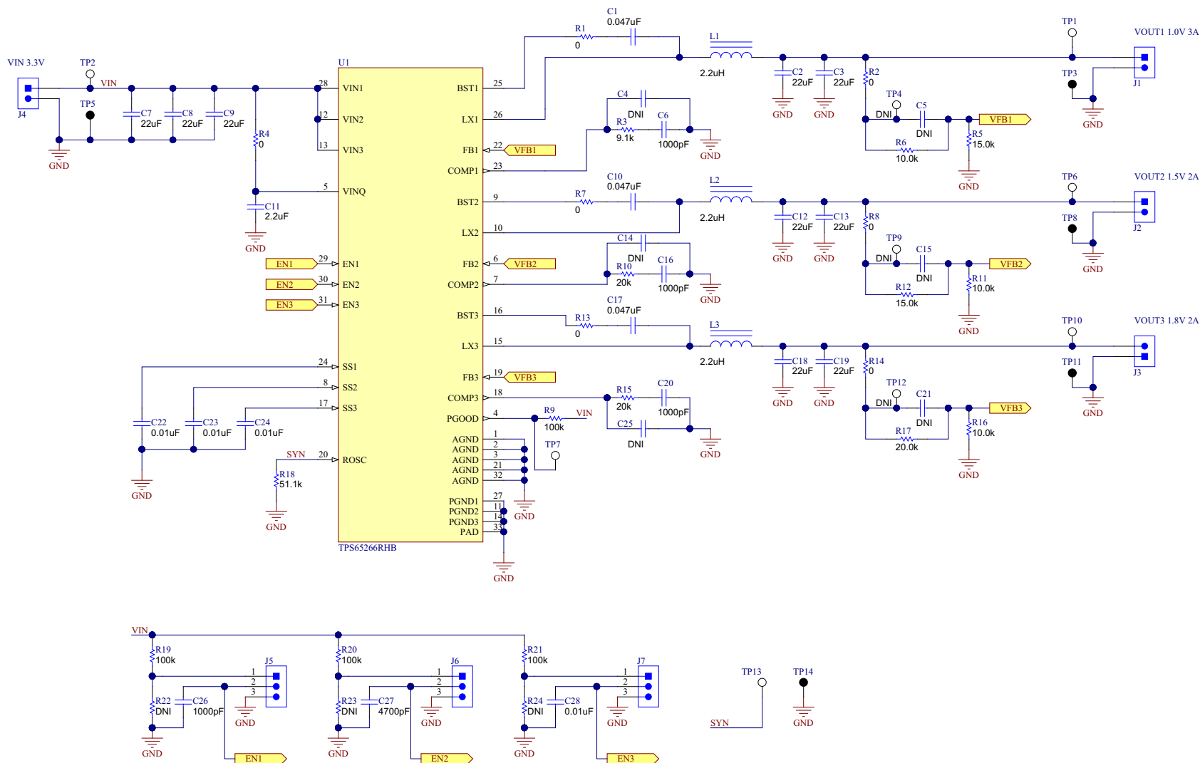
Figure 1. TPS65266EVM-686 Schematic
