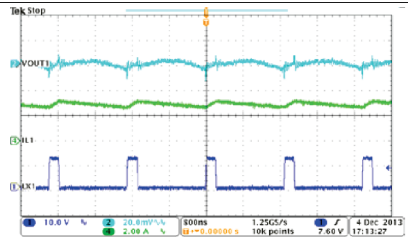
Figure 38. Buck1, Steady State Operation With Full Load
