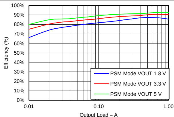
Figure 2. Buck2 Efficiency
