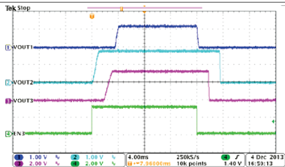
Figure 55. Automatic Power Sequencing, MODE = EN1 = EN2 = HIGH
