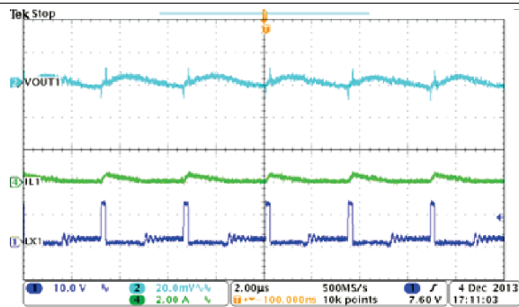
Figure 37. Buck1, Steady State Operation With Light Load
