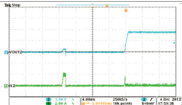
Figure 50. Buck1, Hiccup and Recovery
