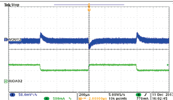
Figure 44. Buck1, Load Transient, 1.5 to 2.25 A SR = 0.25 A/µs
