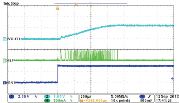
Figure 31. Buck1, Soft-Start With No Load
