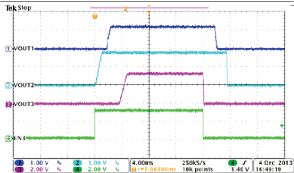
Figure 57. Automatic Power Sequencing, MODE = EN1 = HIGH, EN2 = LOW
