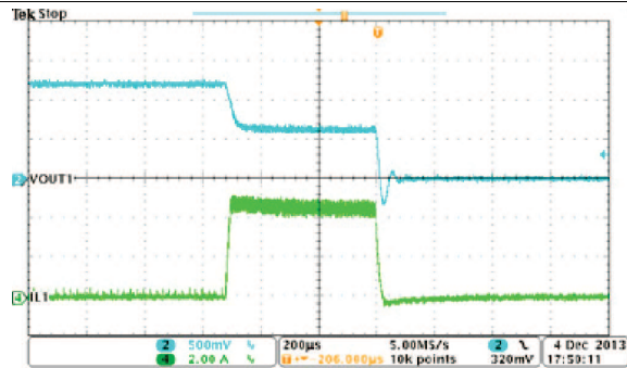
Figure 49. Buck1, Overcurrent Protection
