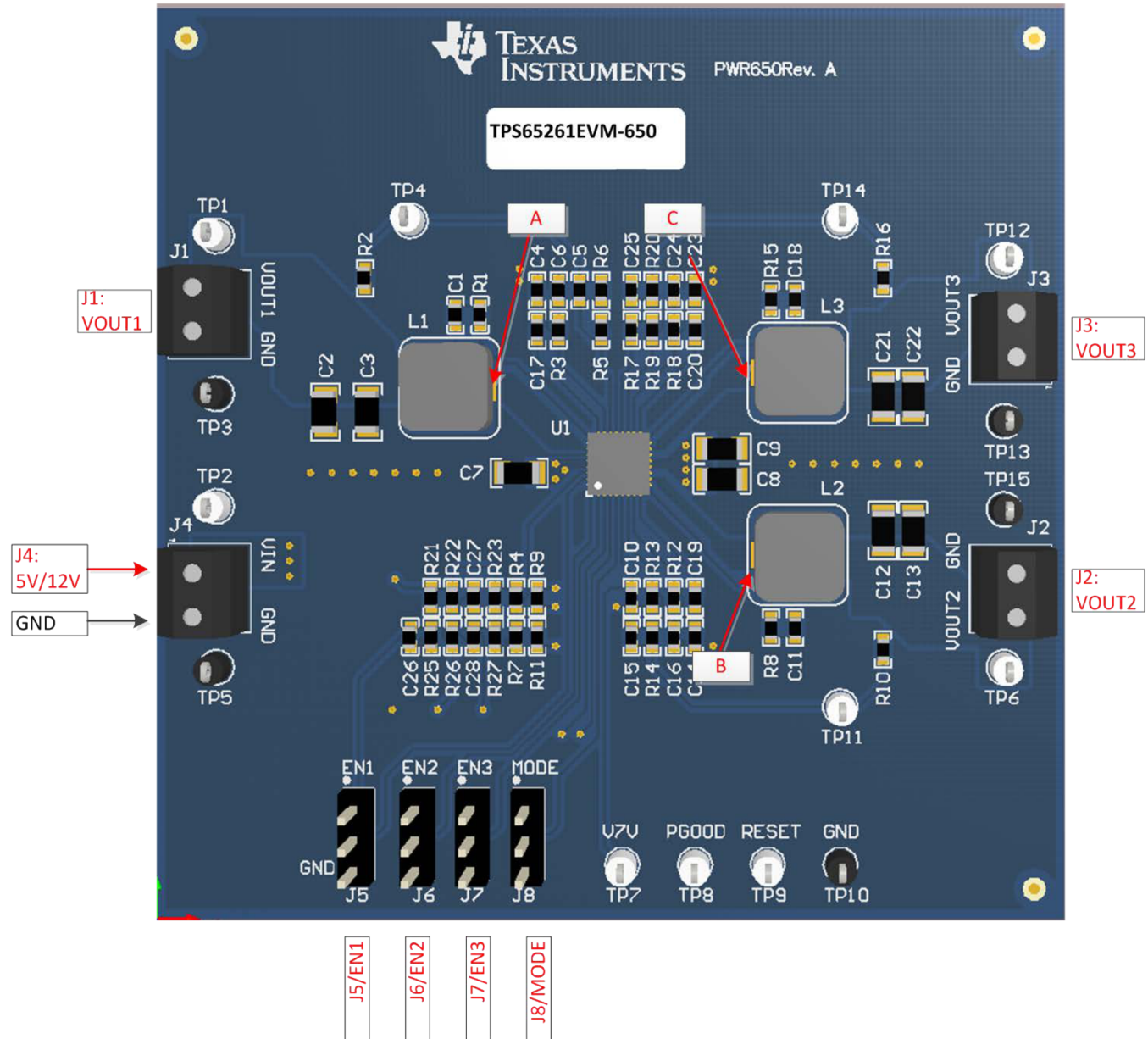
Figure 7. Header Descriptions and Jumper Placement
