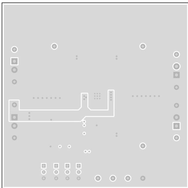
Figure 5. Board Layout (Third Layer)
