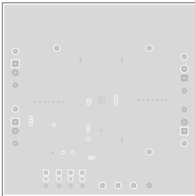
Figure 4. Board Layout (Second Layer)
