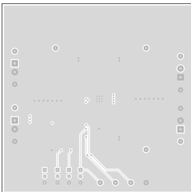
Figure 6. Board Layout (Bottom Layer)
