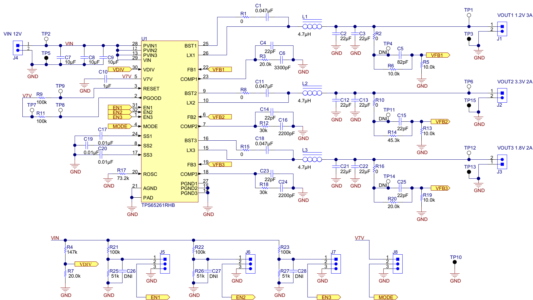
Figure 1. TPS65261 Schematic
