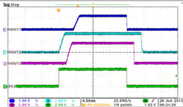
Figure 60. Automatic Power Sequencing, MODE=EN1=EN2=HIGH
