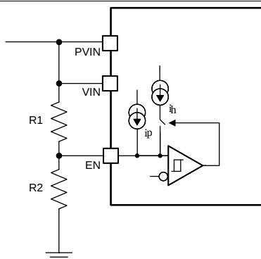
Figure 25. Adjustable VIN and PVIN Under-voltage Lockout
