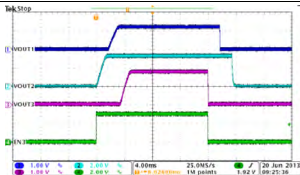
Figure 62. Automatic Power Sequencing, MODE=EN1= HIGH, EN2=LOW
