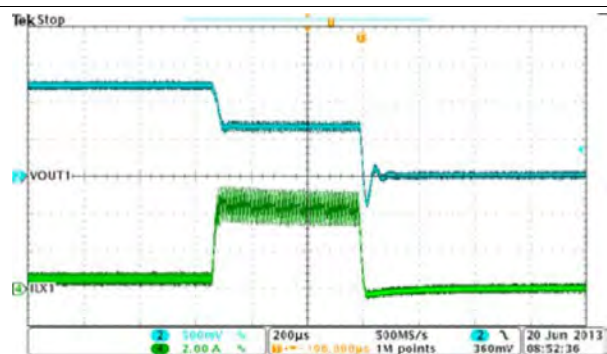
Figure 54. BUCK1, Over Current Protection
