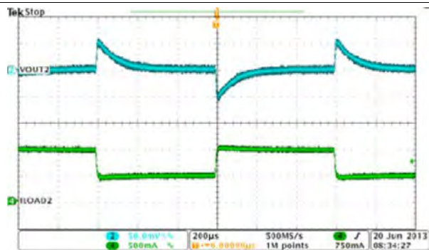
Figure 48. BUCK1, Load Transient, 0.75A to 1.5A SR=0.25A/µs
