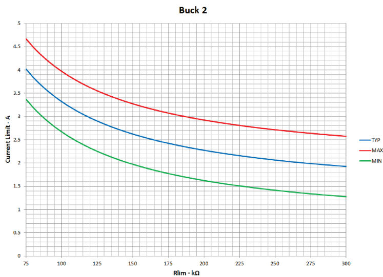
Figure 37. Buck 2
