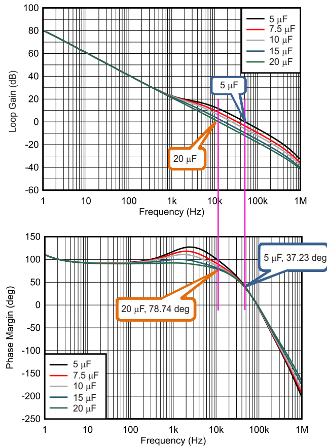
Figure 13. Gain and Phase Margin of the Boost Loop With Different Boost Capacitance (V_{IN} = 12\text{ V}, V_{OUT} = 18.2\text{ V}, I_{LOAD} = 1\text{ A}, F_{SW} = 1\text{ MHz}, 10\text{ }\mu\text{H}, \text{Typical Bode Plot})
