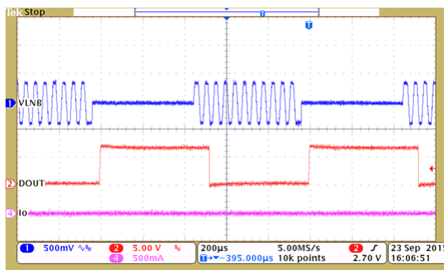
Figure 39. DOUT Tone Detection Output
