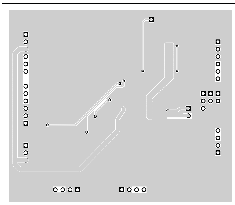
Figure 4. Bottom Layer
