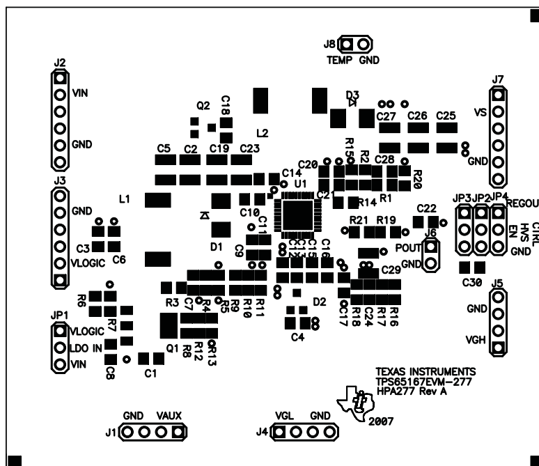
Figure 2. Top Assembly
