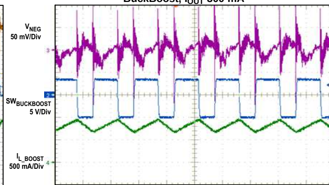
400 ns/div Figure 6.
