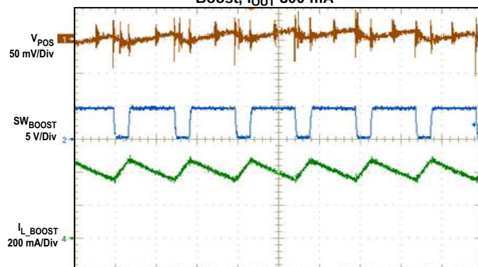
400 ns/div Figure 5.
