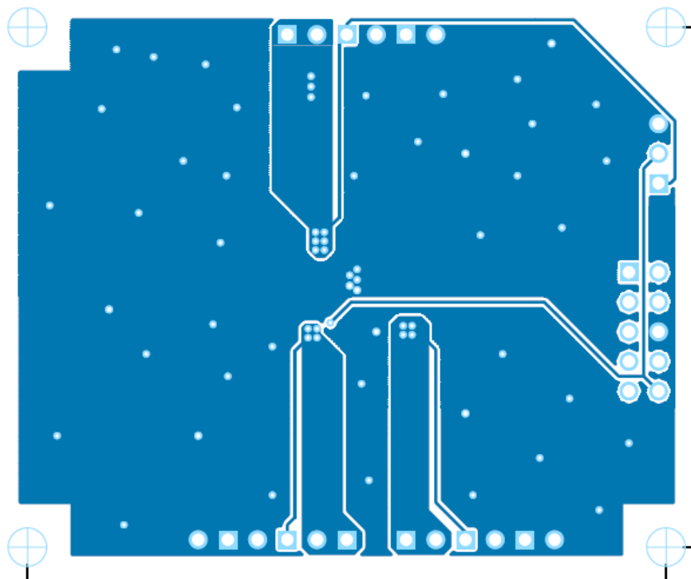
Figure 11. Example of Board Layout. Bottom Layer
