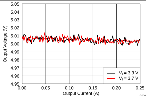
Figure 13. V_{POS} Load Regulation
