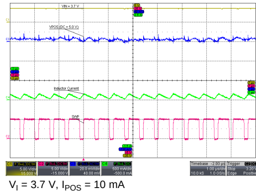
Figure 19. V_{POS} Switching Waveforms (10 mA)
