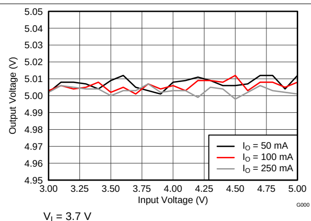
Figure 11. V_{\text{POS}} Line Regulation
