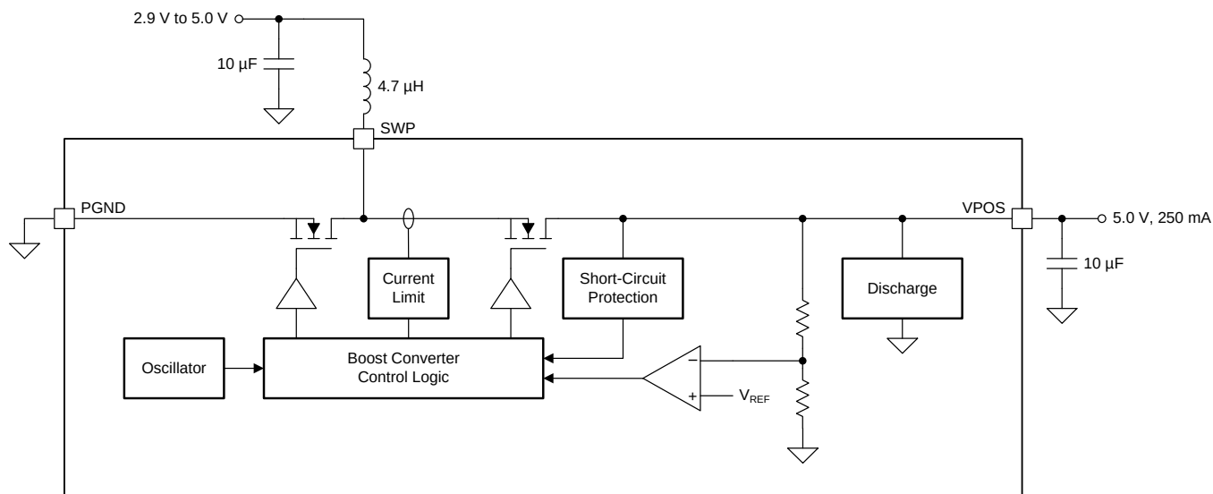
Figure 6. V_{POS} Boost Converter Internal Block Diagram
