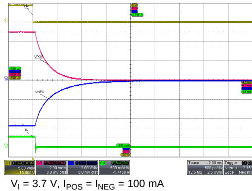
Figure 18. V_{POS} and V_{NEG} Shutdown Behavior (100 mA)
