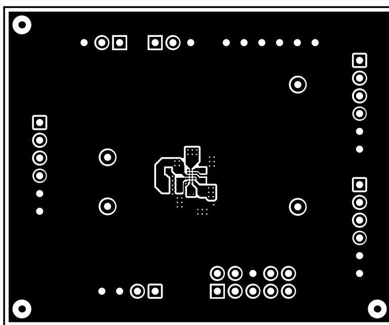
Figure 16. PCB Top Layer (Top View)
