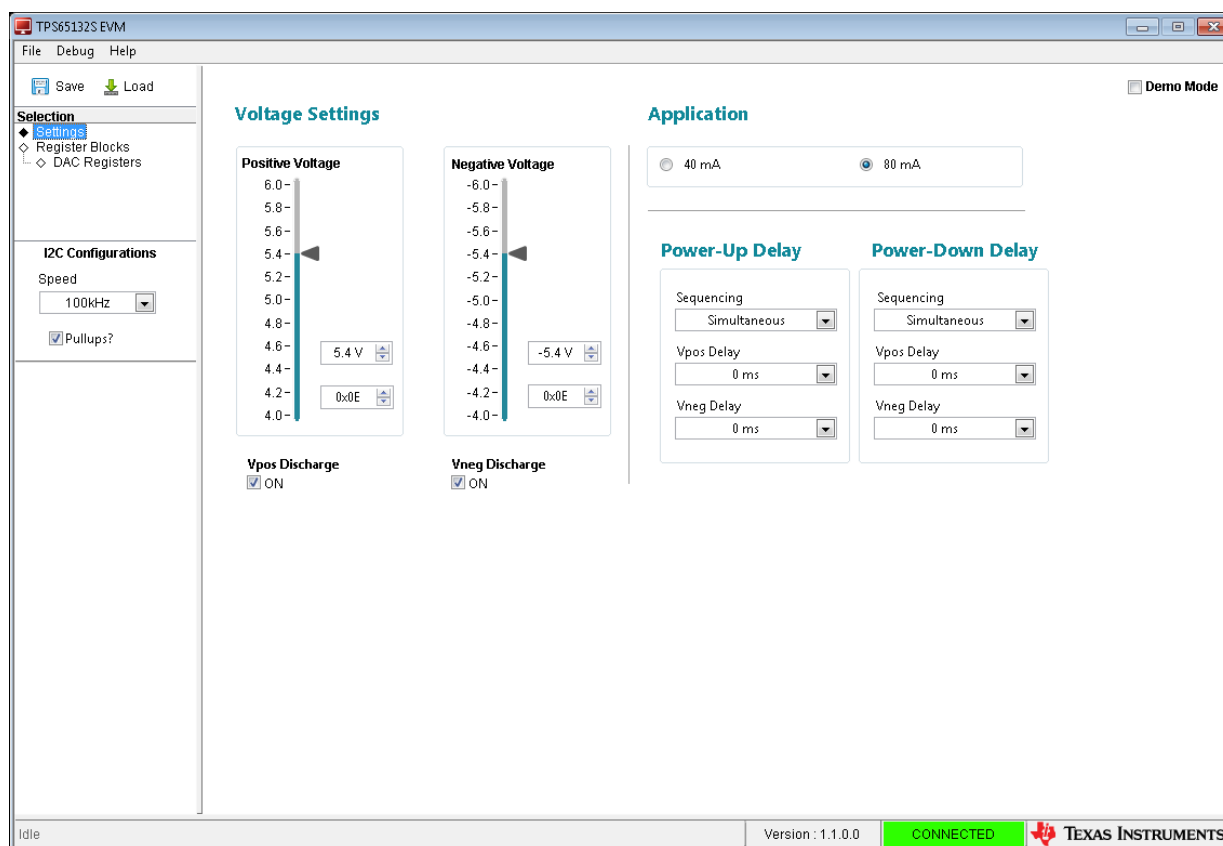
Figure 10. Settings Window
