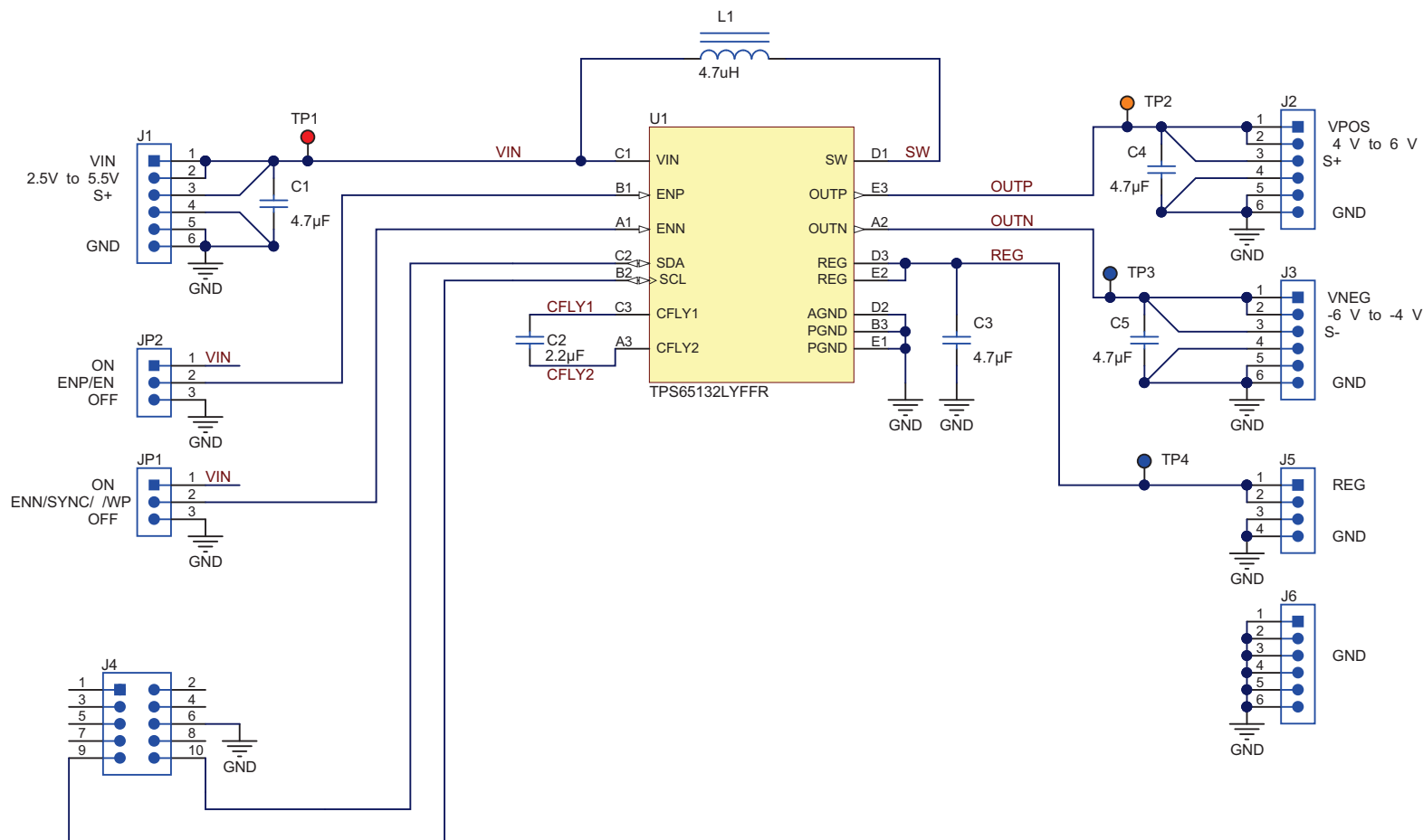
Figure 1. Schematic
