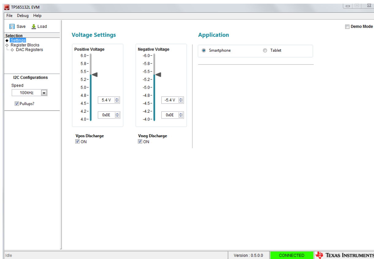
Figure 10. Settings Window
