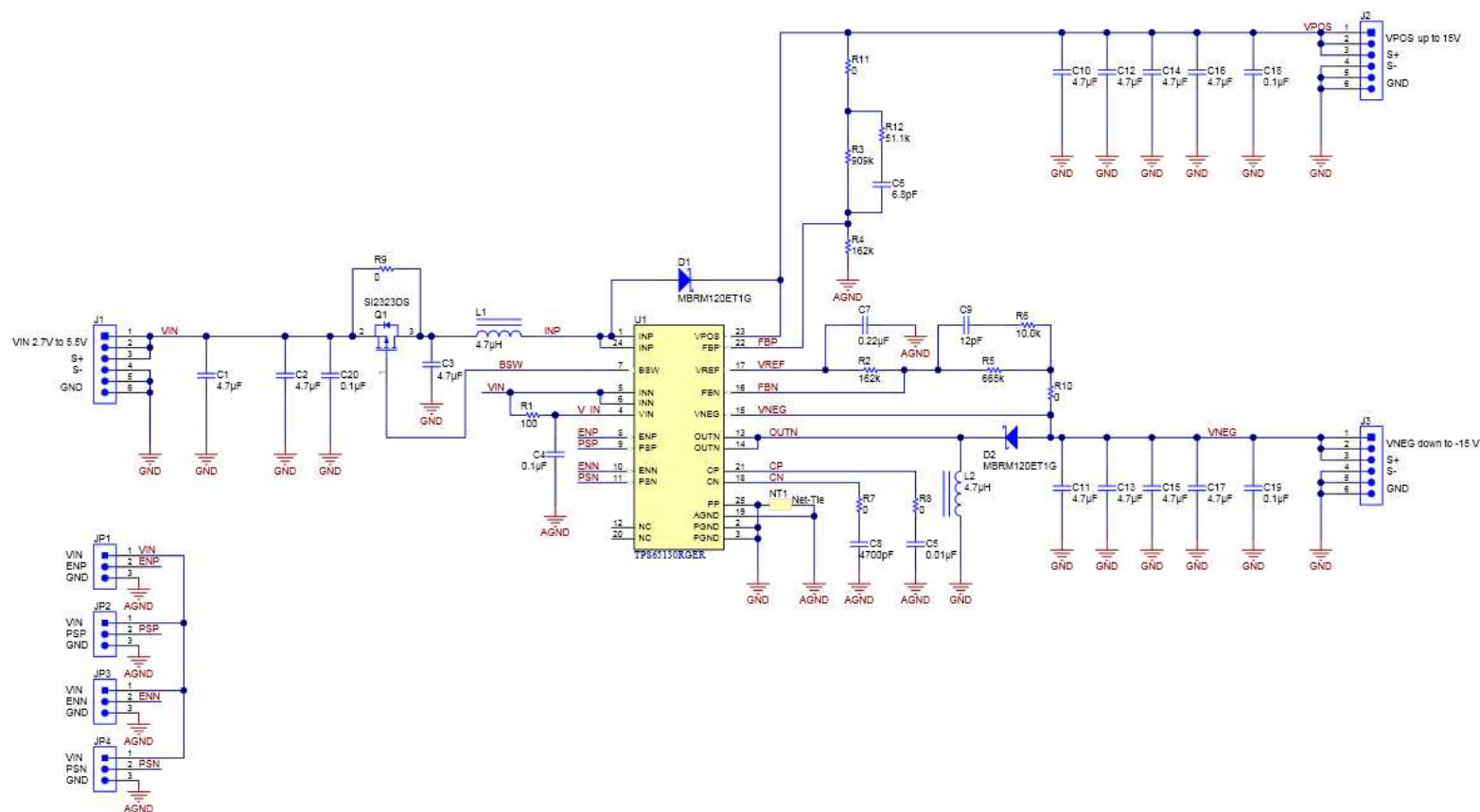
Figure 1. TPS65130EVM-839 Schematic
