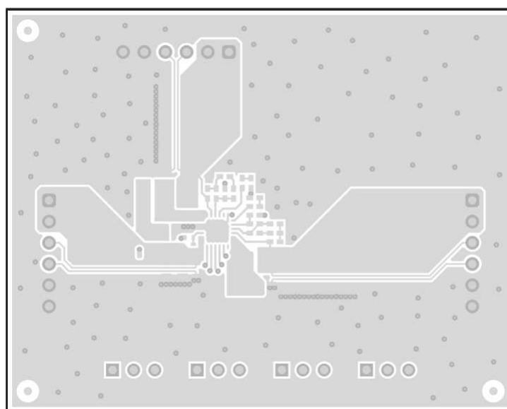
Figure 5. Top Layer
