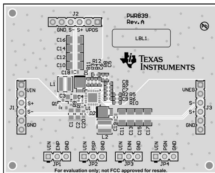
Figure 4. Top Assembly Layer
