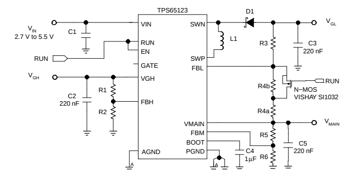
Figure 23. Complete TFT-LCD Power Supply from 1 cell Li-Ion
