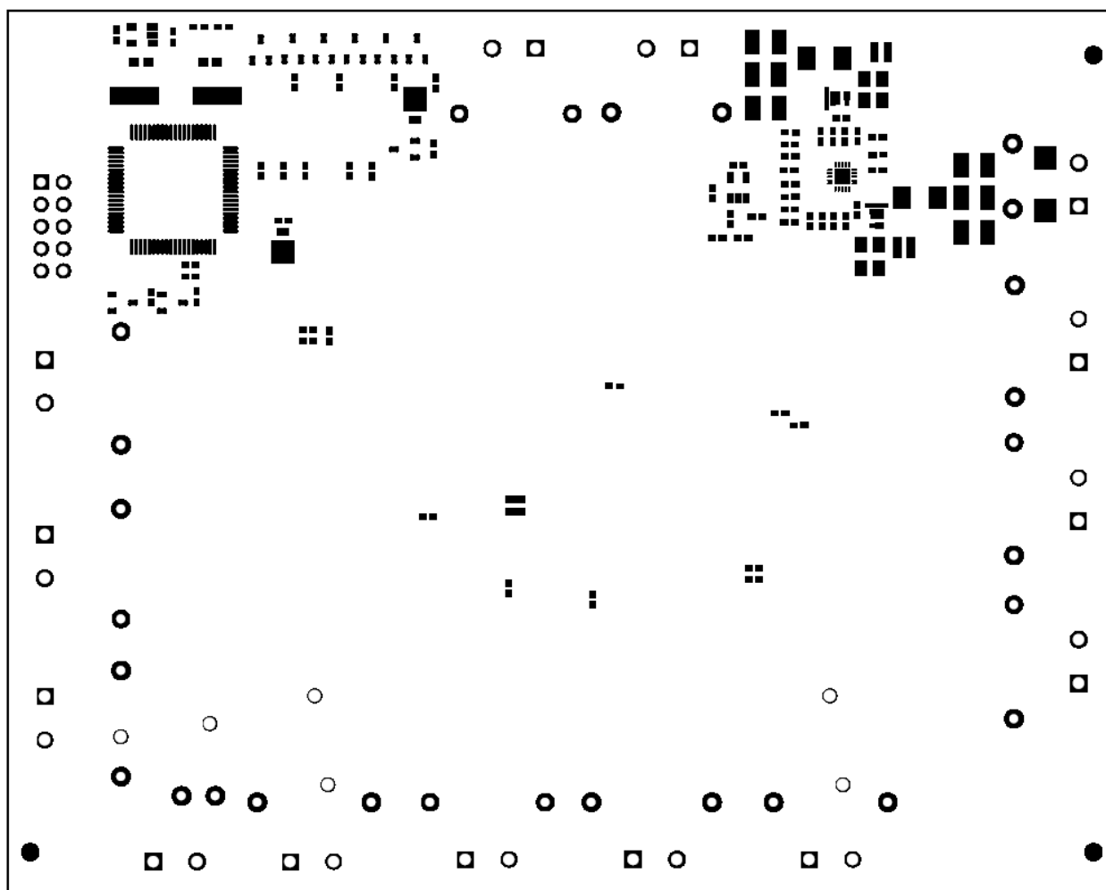
Figure 22. Bottom Solder Mask
