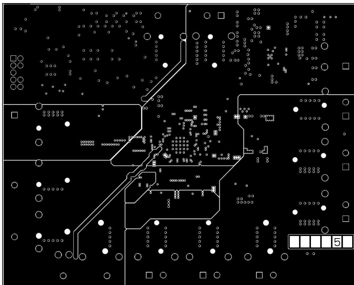
Figure 20. Power Layer
