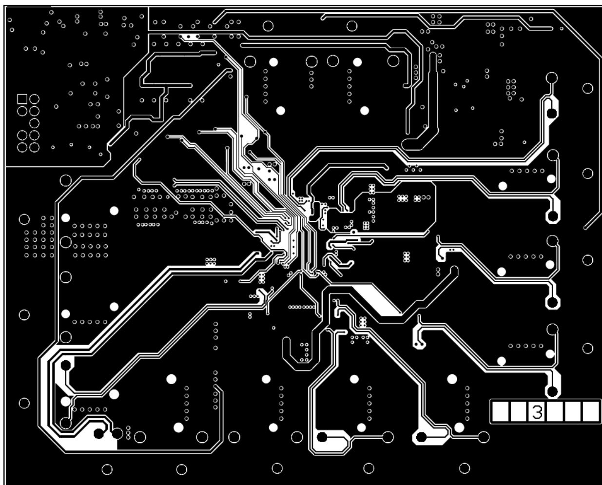
Figure 18. Signal Layer 1
