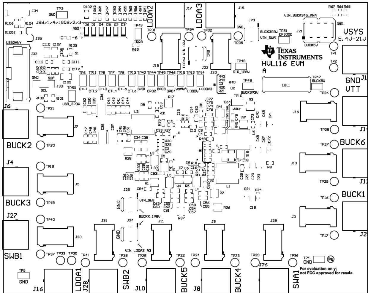
Figure 14. Top Overlay
