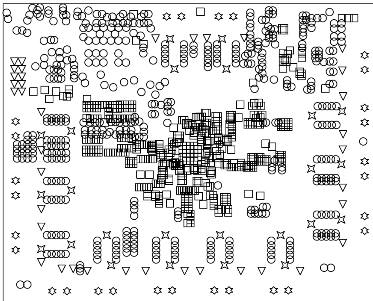
Figure 24. Drill Drawing
