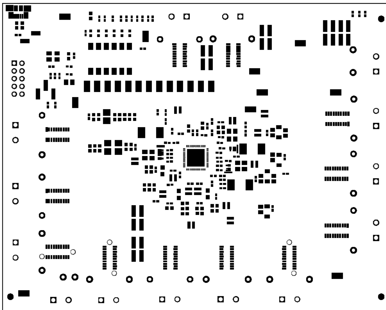
Figure 15. Top Solder Mask
