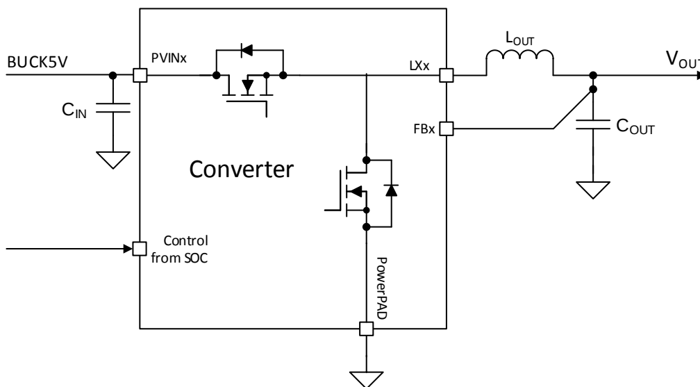
Figure 6-3. Converter Diagram
