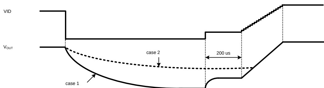
Figure 5-7. Decay Down to 0 V and Slew Up
