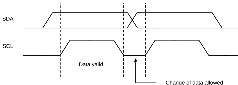
Figure 5-14. Bit Transfer on the I 2 C Bus
