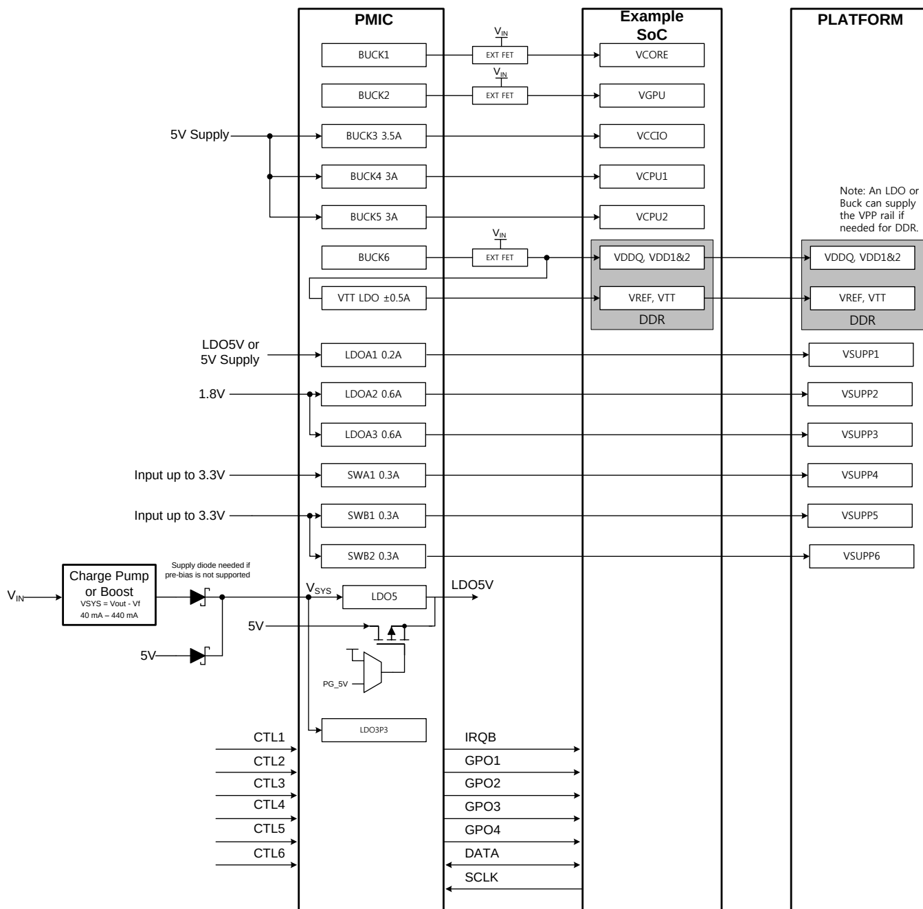
Figure 6-6. VIN 5-V Application
