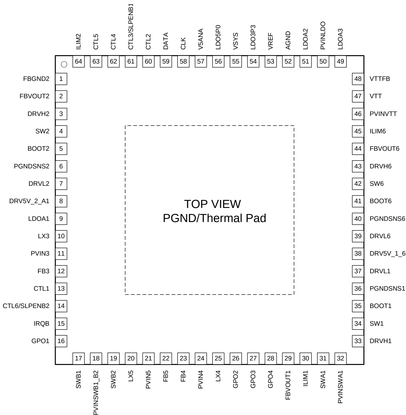
Figure 3-1. RSK (VQFN) Pin Map Diagram
