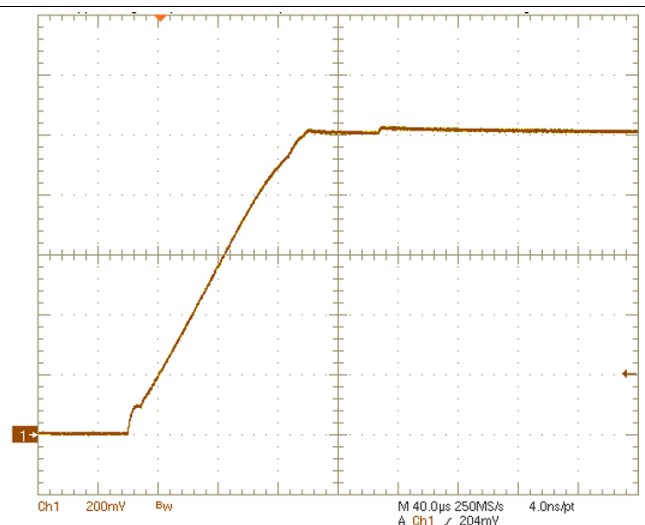
Figure 4-2. BUCK3 Converter Start Up
