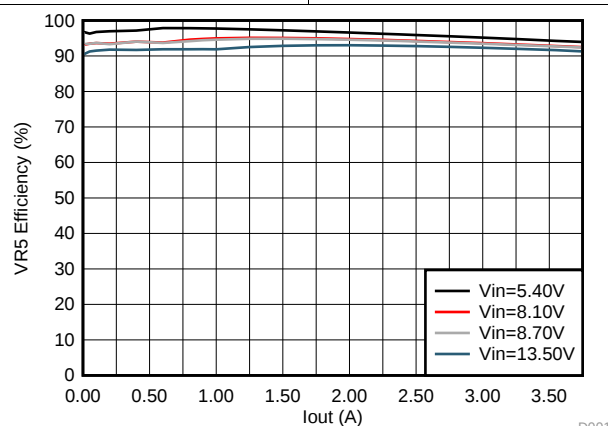
Figure 7-17. Typical Efficiency for VR5
