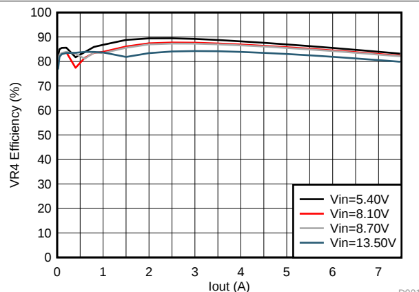
Figure 7-16. Typical Efficiency for VR4
