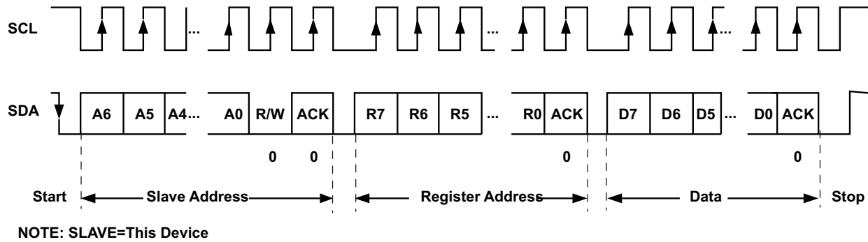
Figure 6-21. I²C Interface WRITE to Device in F/S Mode
