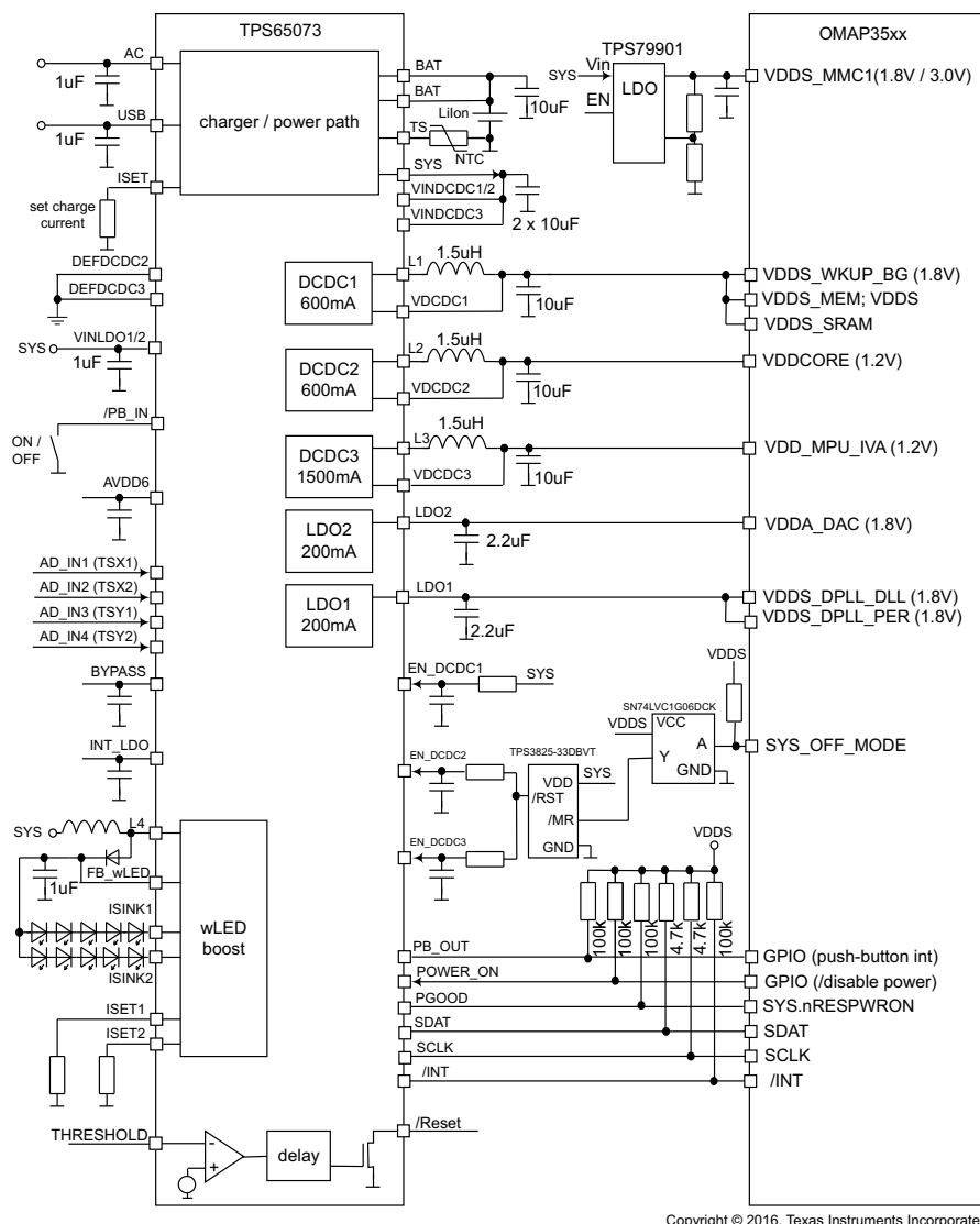
Figure 56. OMAP35xx (Supporting SYS-OFF Mode)
