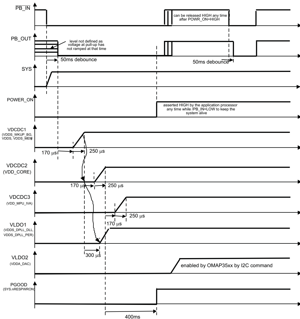
Figure 59. TPS650731: OMAP35xx Sequence
