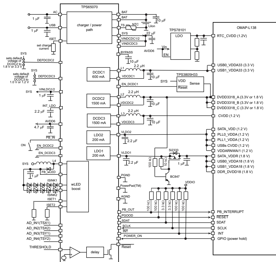
Figure 50. Powering OMAP-L138
