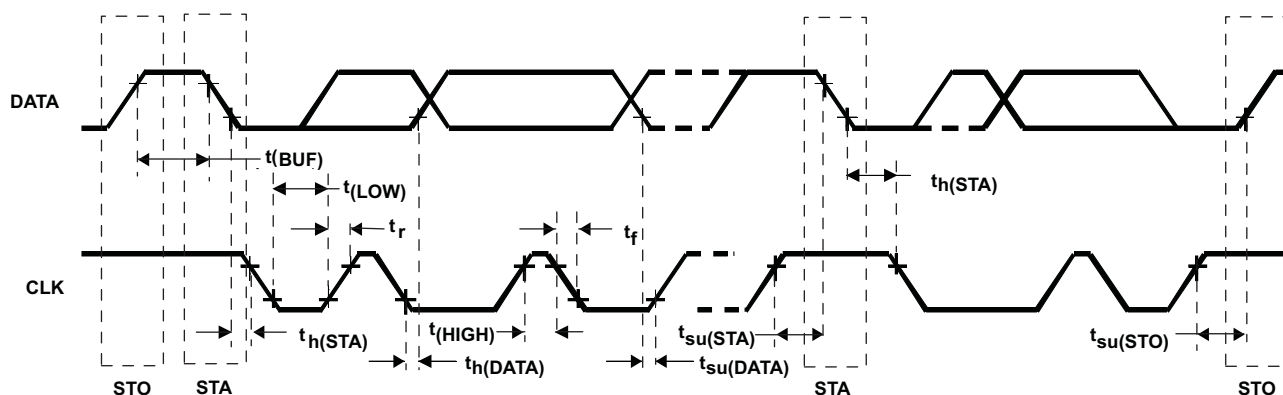
Figure 1. Serial Interface Timing Diagram
