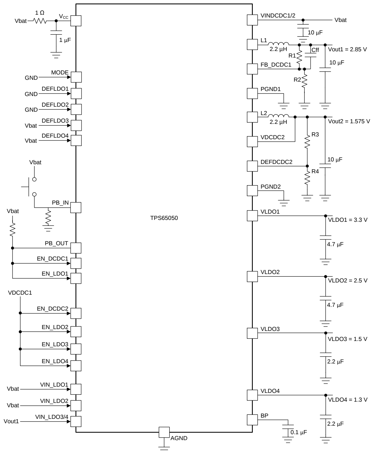
Figure 15. Typical Example Application With PB_ON/OFF Circuit
