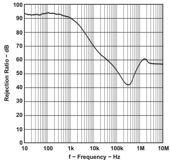
Figure 5. Power Supply Rejection Ratio vs Frequency
