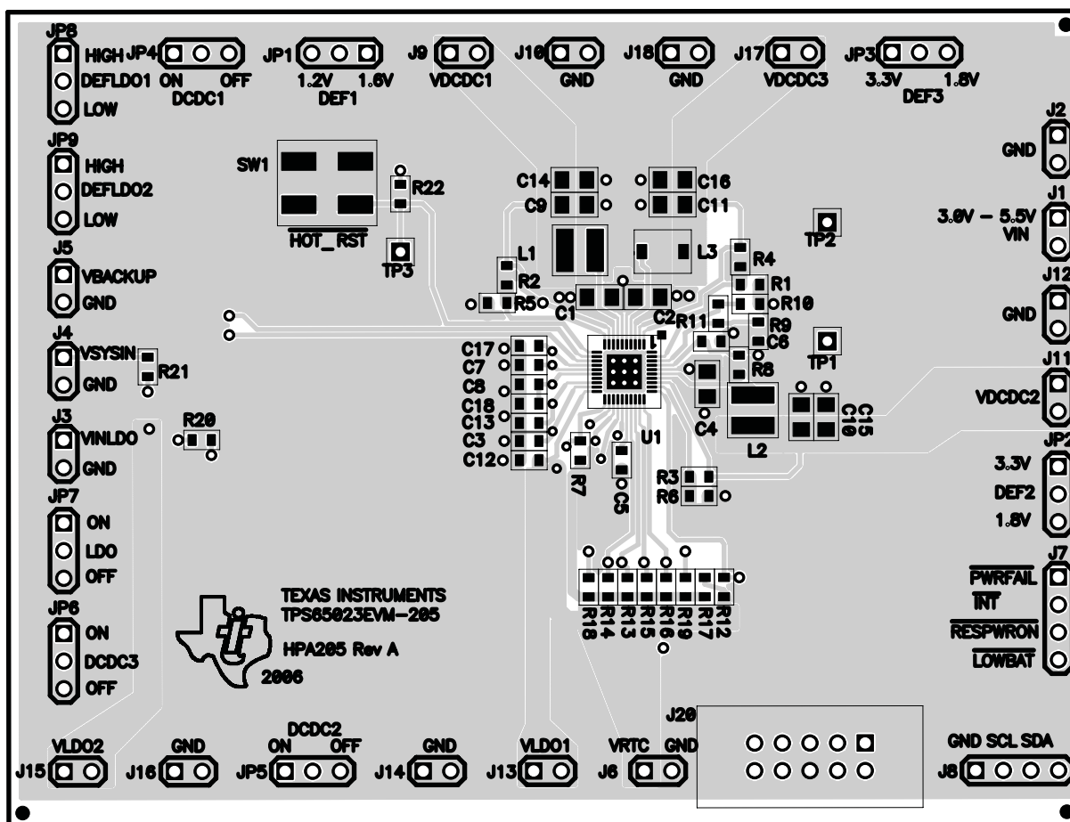
Figure 1. Assembly Layer
