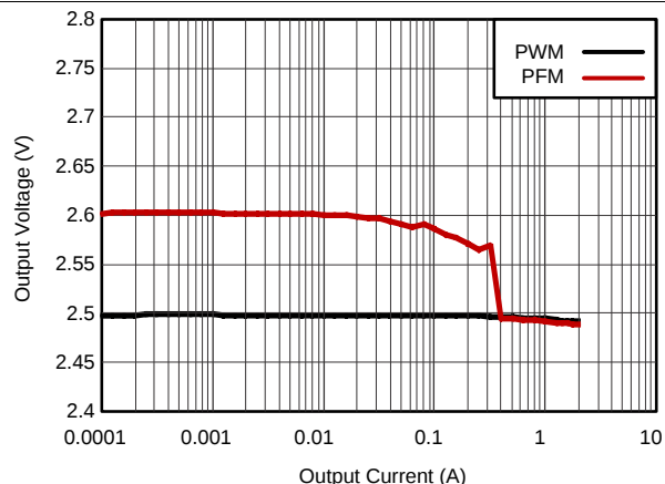
TPS63060 V_{OUT} = 2.5\text{ V} Power Save Disabled V_{IN} = 7.2\text{ V}
