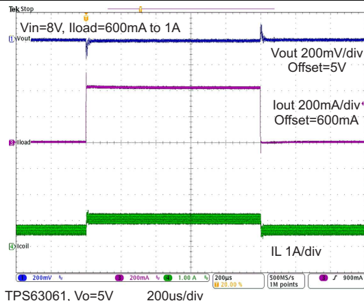
TPS63061, V_o=5\text{ V} 200us/div
