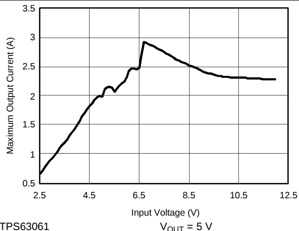
Figure 10. Output Current vs Input Voltage
