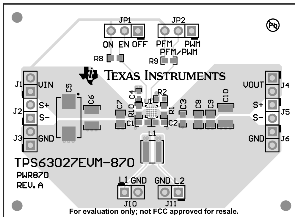
Figure 1. Assembly Layer
