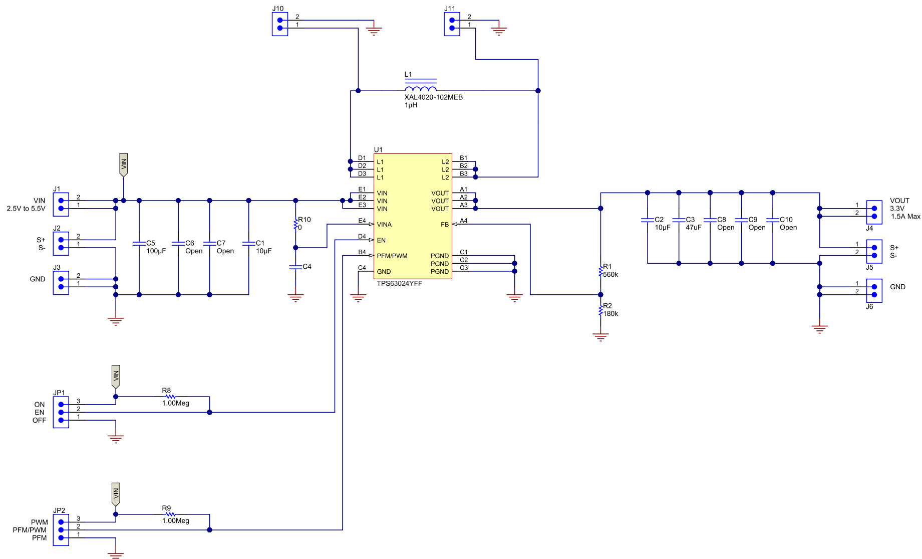
Figure 4. TPS63024xEVM-553 Schematic
