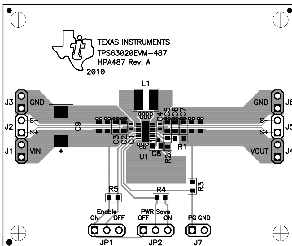
Figure 6. Assembly Layer
