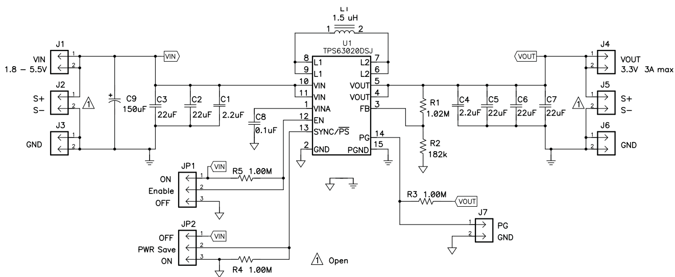
Figure 9. Schematic
