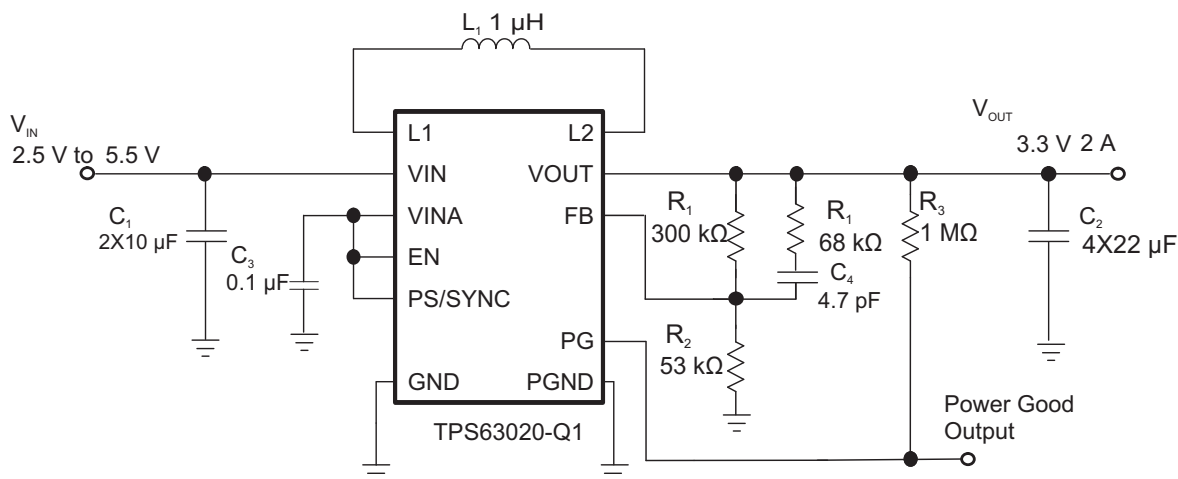
Figure 18. Application Circuit for 2-A Load Current
