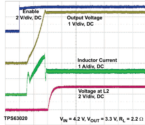
Figure 27. Start-up Behavior from Rising Enable, TPS63020
