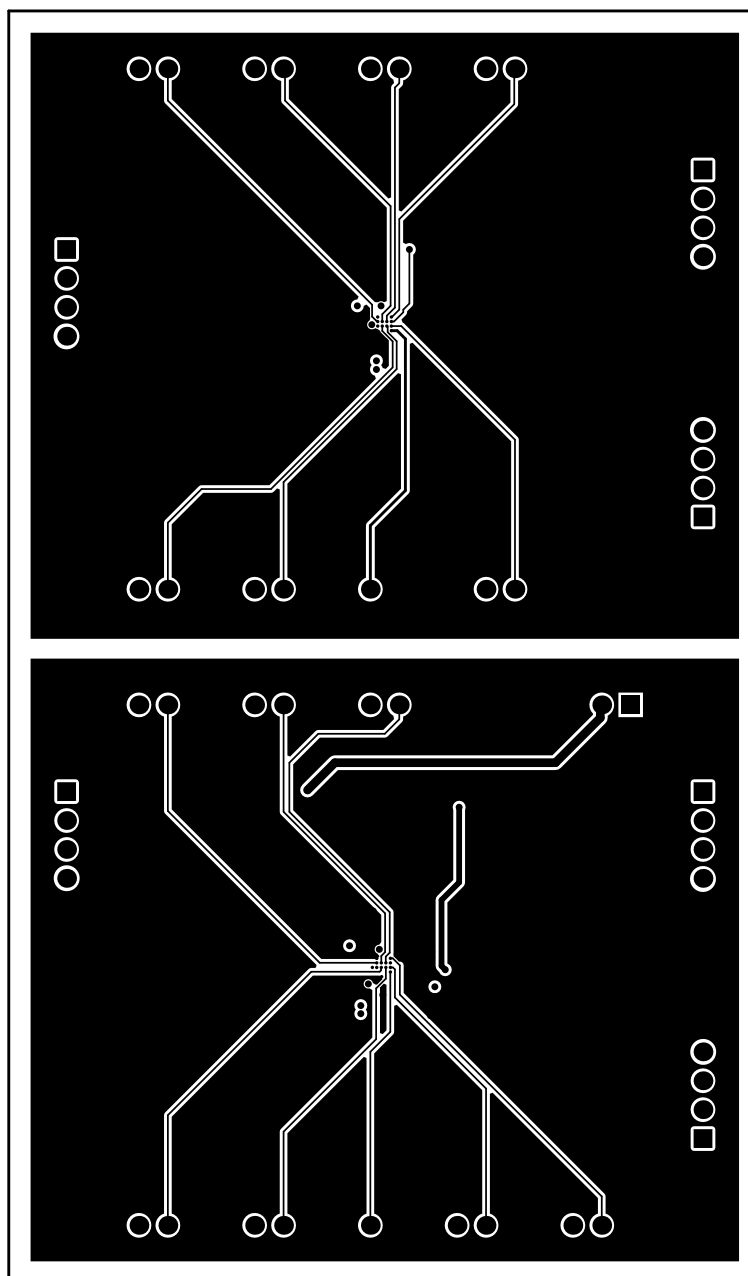
Figure 4. Signal 2 Layer
