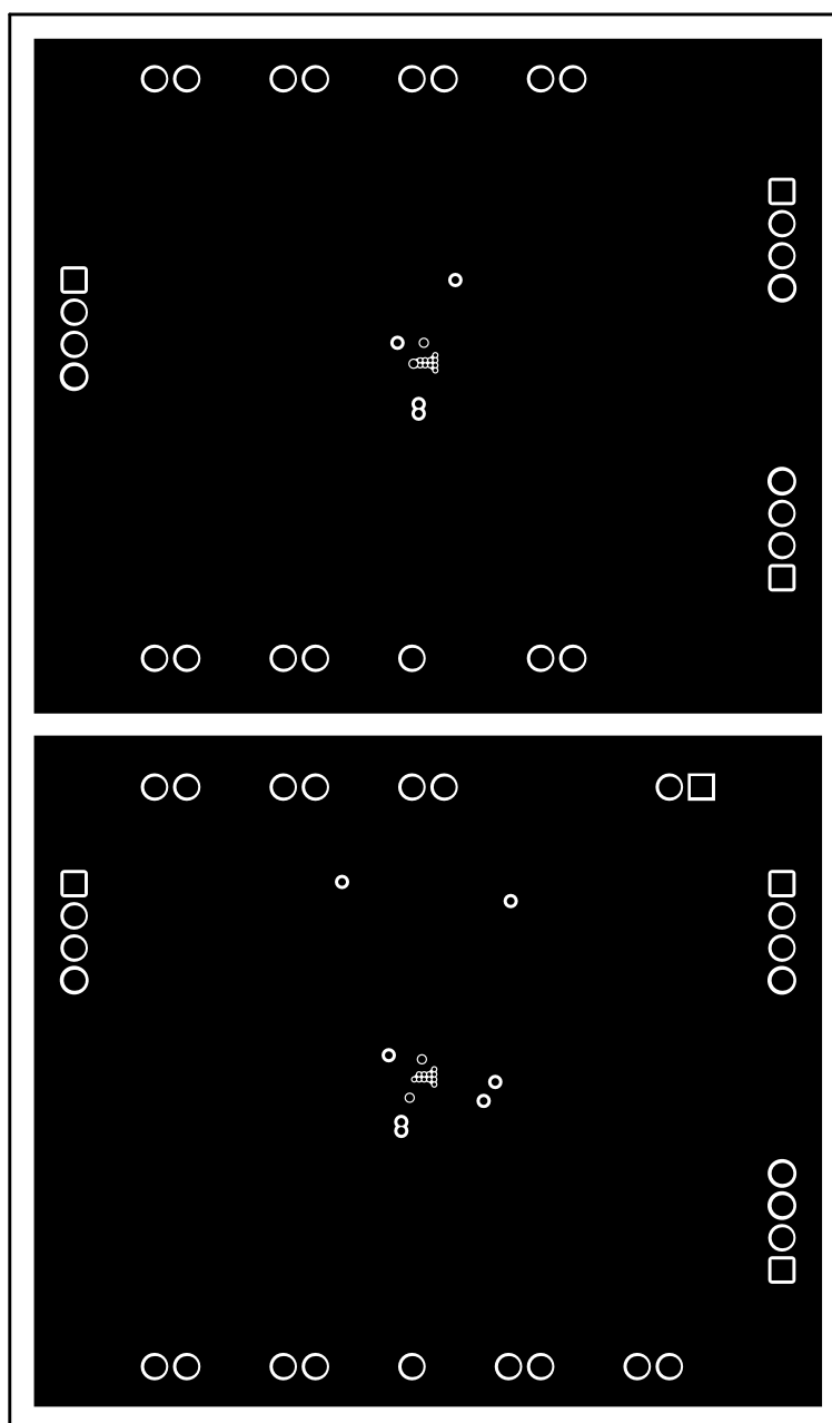
Figure 3. Signal 1 Layer
