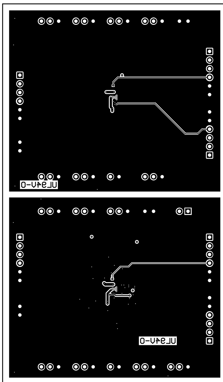
Figure 5. Bottom Layer
