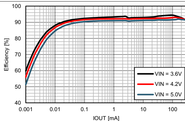
Figure 11. Efficiency vs. IOUT, VOUT1 = 1.2 V
