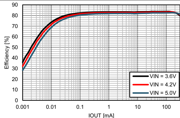
Figure 10. Efficiency vs. IOUT, VOUT1 = 1.0 V
