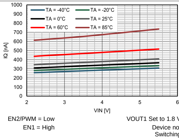
Figure 1. Quiescent Current I_Q Step-Down converter
