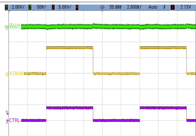
Figure 27. VINSW Operation and Control
