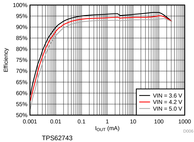
Figure 8. Efficiency vs Load Current, V_{OUT} = 3.3\text{ V}
