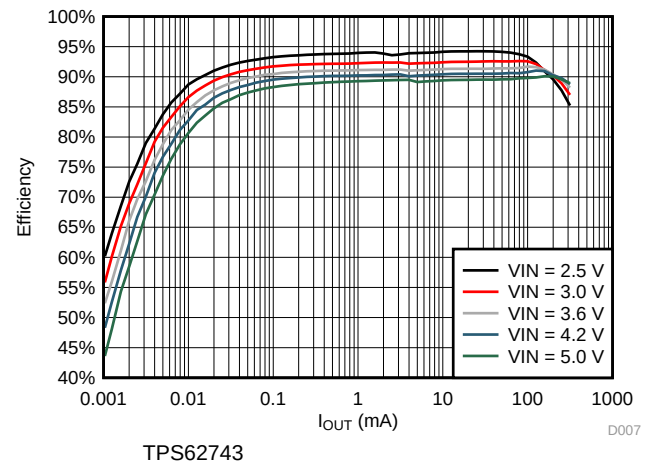
Figure 9. Efficiency vs Load Current; V_{OUT} = 2.1\text{ V}
