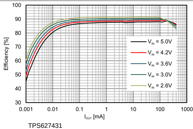
Figure 10. Efficiency vs Load Current; V_{OUT} = 1.9\text{ V}
