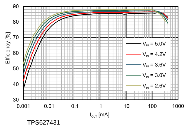
Figure 12. Efficiency vs Load Current; V_{OUT} = 1.4\text{ V}
