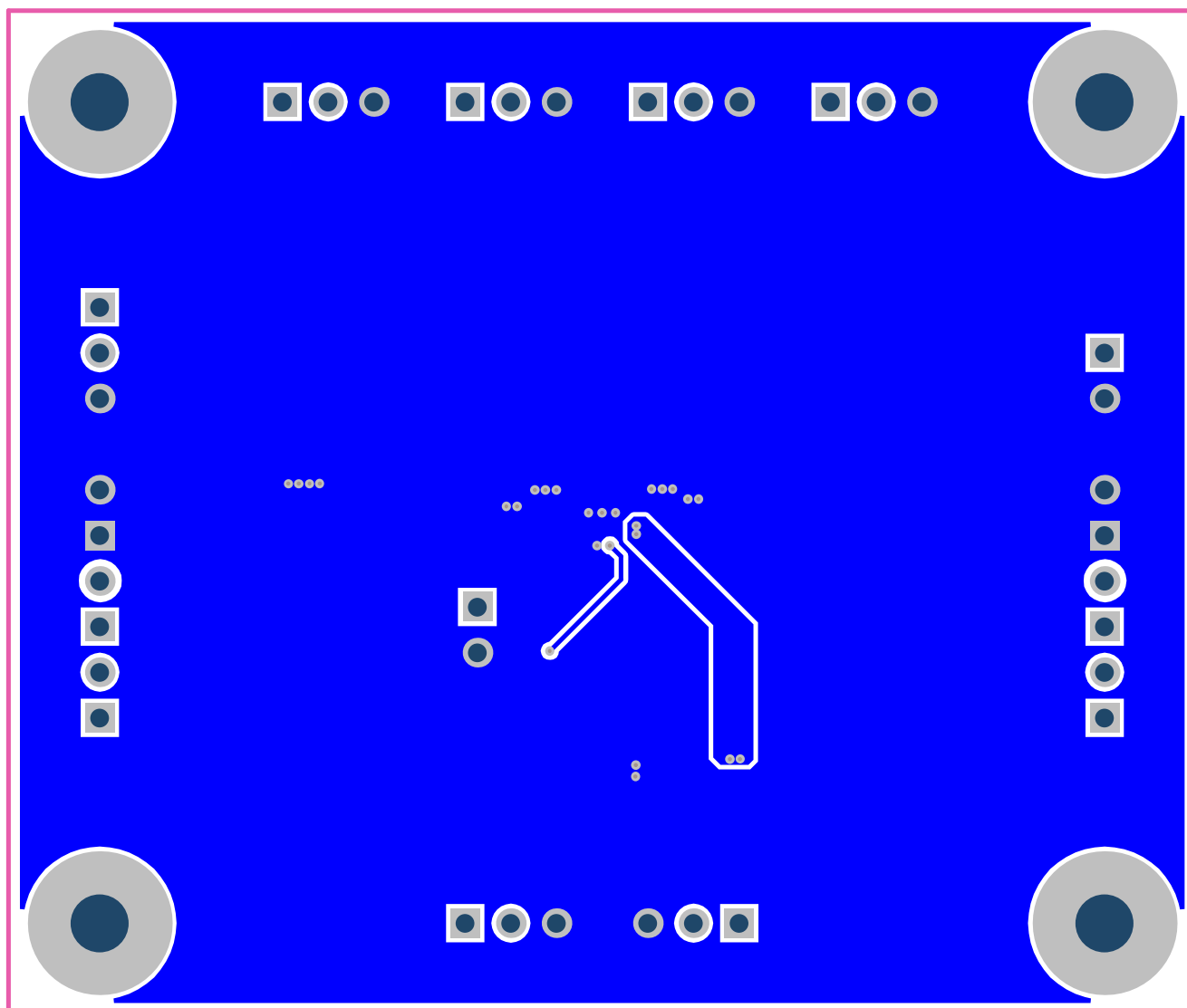
Figure 3. Bottom Layer
