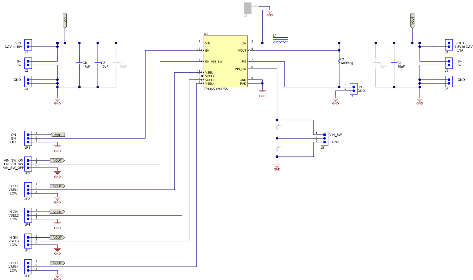
Figure 4. TPS62745EVM-622 Schematic
