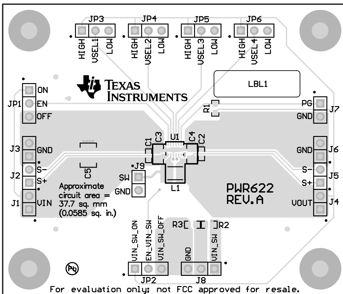
Figure 1. Assembly Layer
