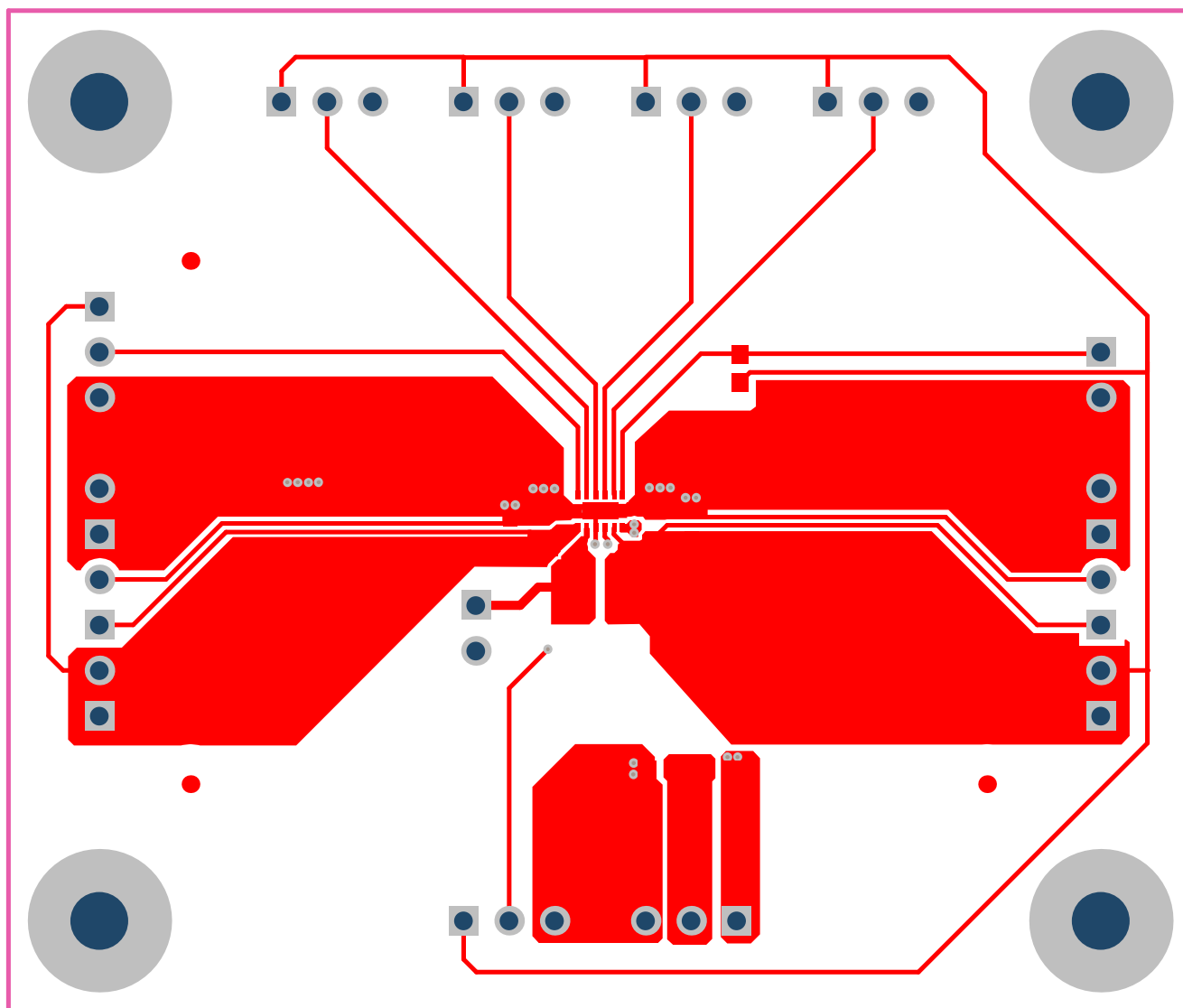
Figure 2. Top Layer
