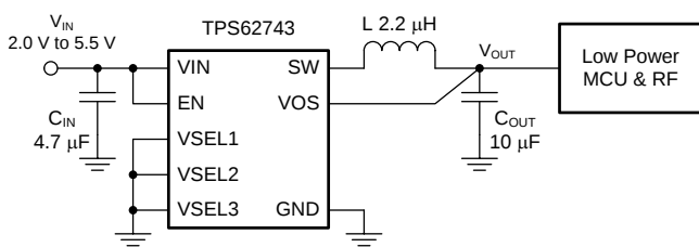
Typical Application
