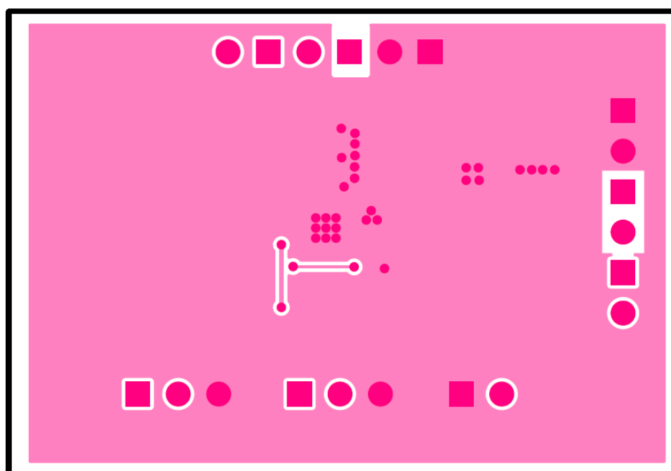
Figure 13. Bottom Layer
