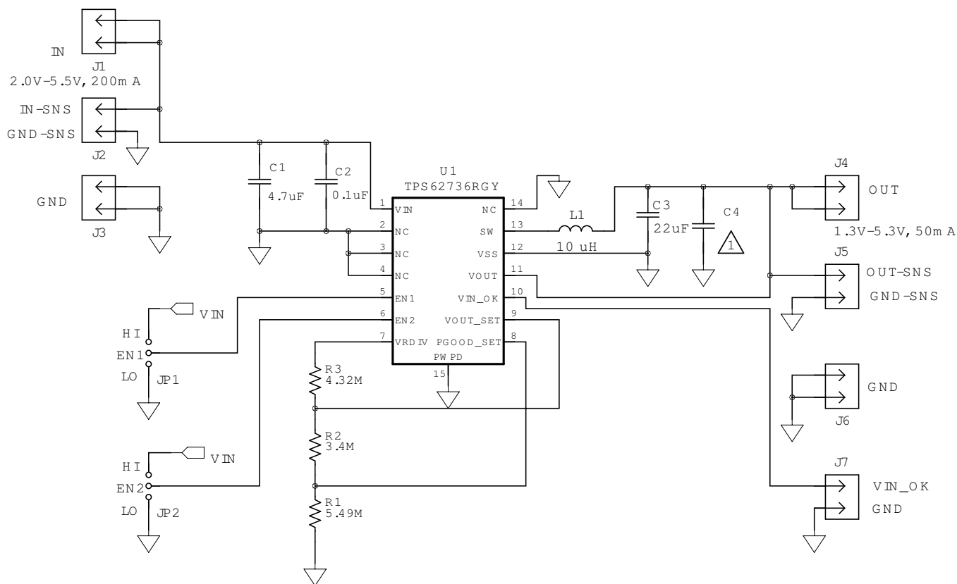
Figure 1. TPS62730 and TPS62733 EVM Board Schematic
