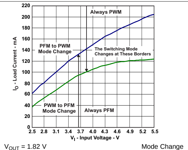
Figure 29. PFM/PWM Boundaries, V_{OUT} = 1.82 V
