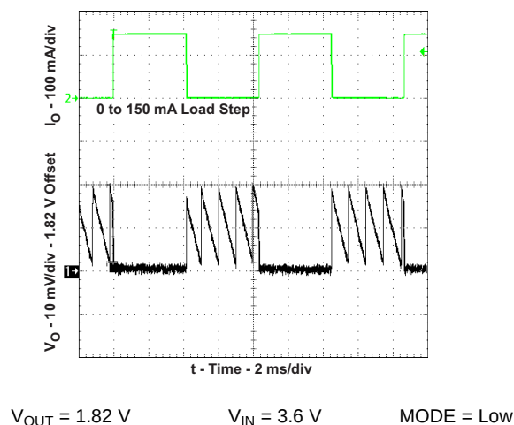
Figure 15. Load Transient Response in PFM/PWM Operation, V_{OUT} = 1.82 \text{ V} , V_{IN} = 3.6 \text{ V}
