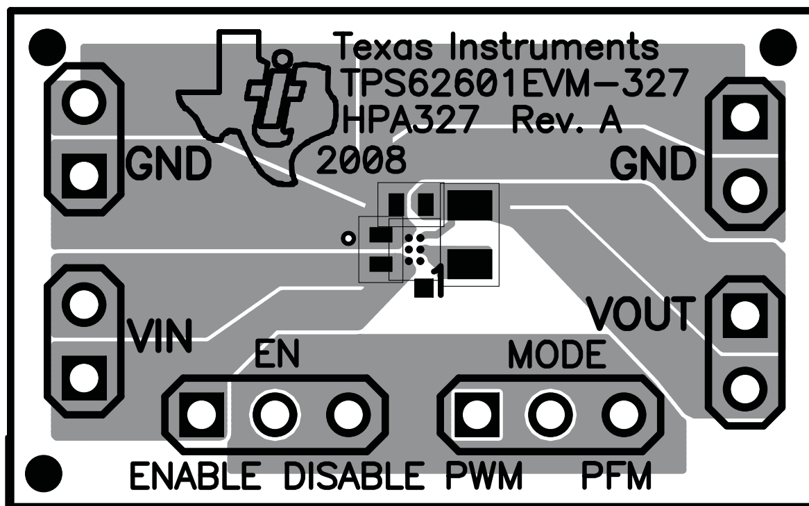
Figure 1. Assembly Layer
