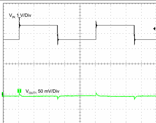
Time base – 400 \mu s/Div MODE/DATA = low V_{IN} = 3.6 to 4.6 V V_{OUT1} = 1.575 V I_{OUT1} = 200 mA
