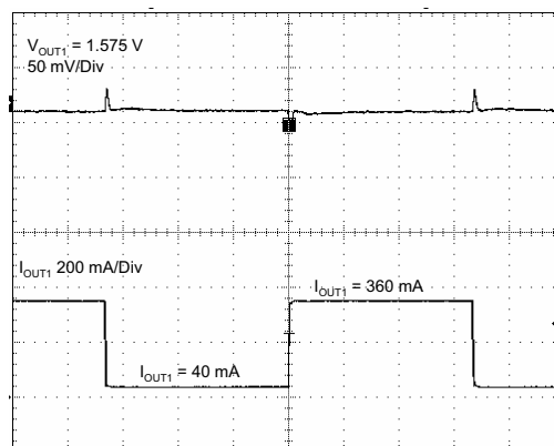
Time base – 50 \mu s/Div PWM mode MODE/DATA = high
