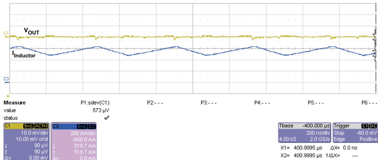
Figure 6. TPS62260 Output Ripple, V_{in} = 3\text{ V} , V_{out} = 1.8\text{ V} , I_{Load} = 600\text{ mA}
