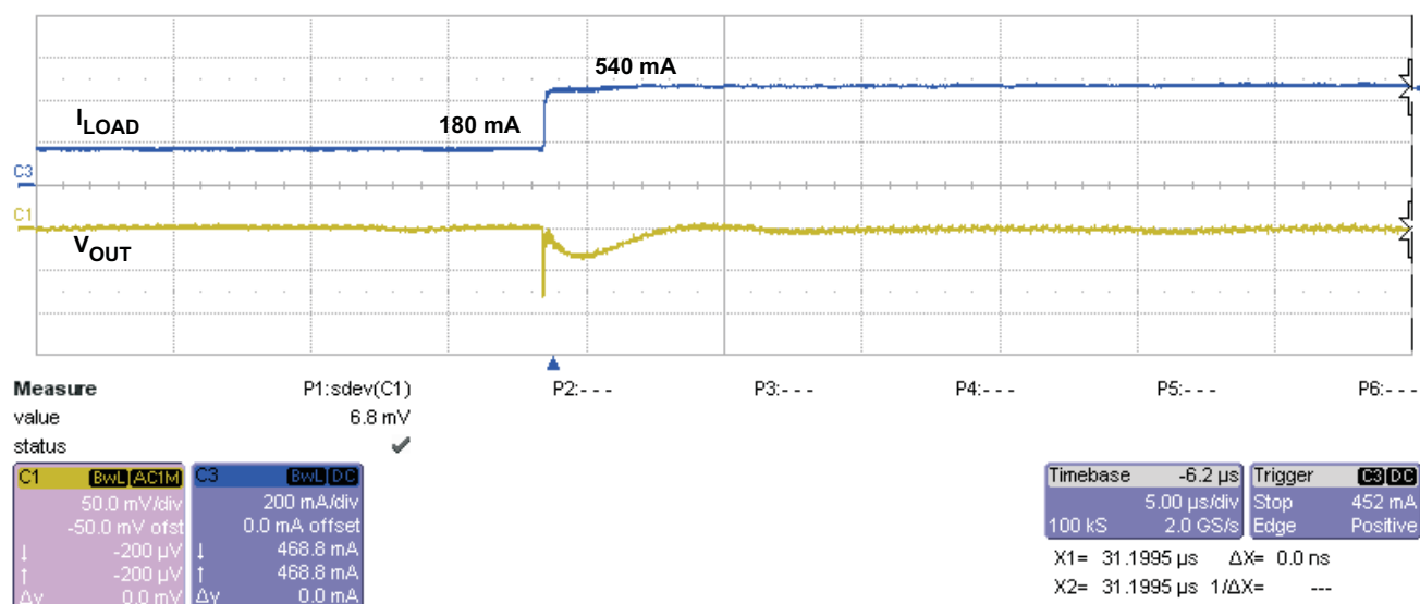
Figure 7. TPS62260 Load Transient, 180-mA to 540-mA Step, V_{in} = 3\text{ V} , V_{out} = 1.8\text{ V}
