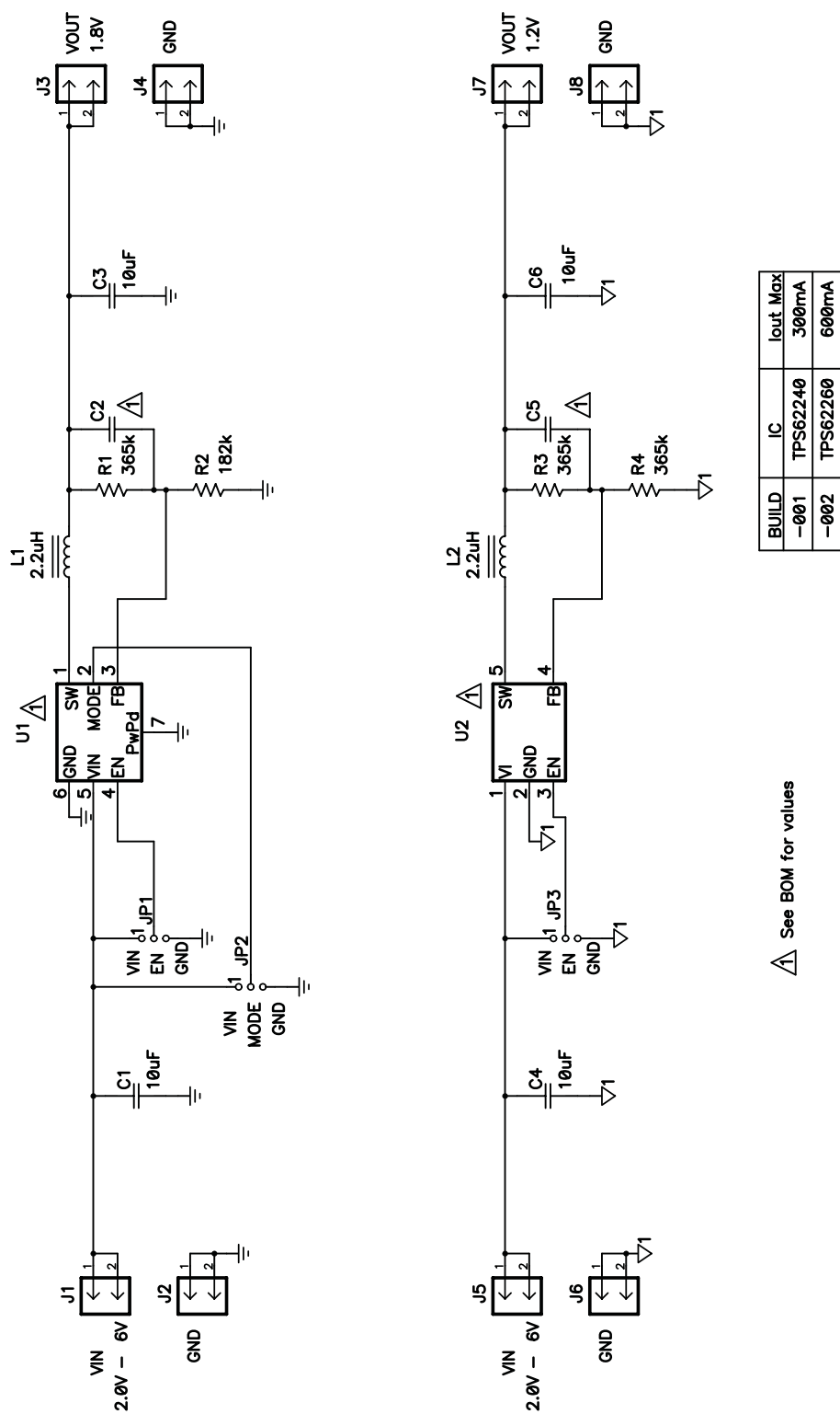
Figure 12. TPS622x0EVM-229 Schematic
