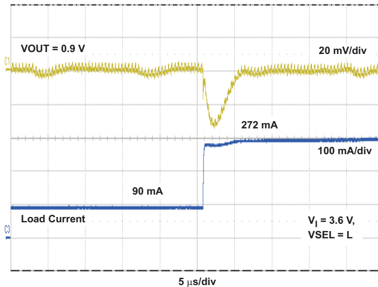
Figure 5. Load Transient, 90 mA to 272 mA step, V_I = 3.6 \text{ V} , VOUT = 0.9 \text{ V}
