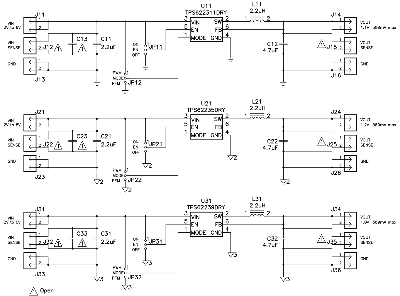
Figure 4. TPS62239EVM-574 Schematic
