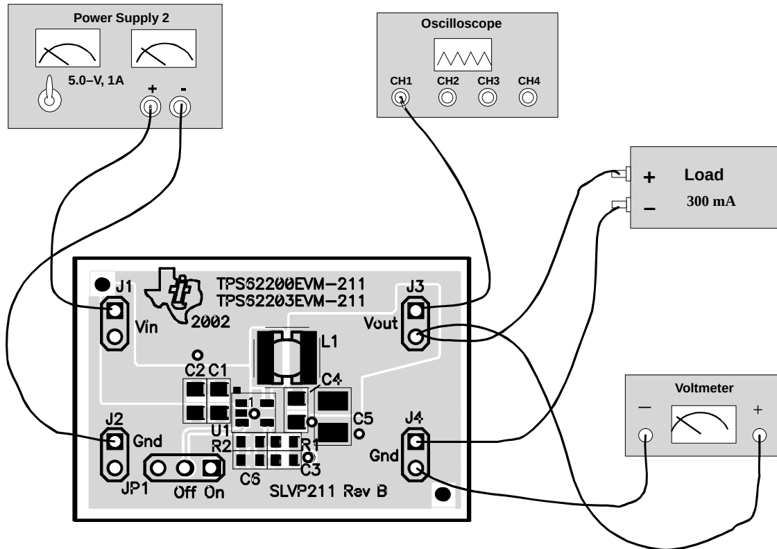
Figure 2–1. Connection Diagram
