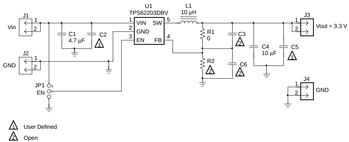
Figure 4–2. TPS62203 Schematic
