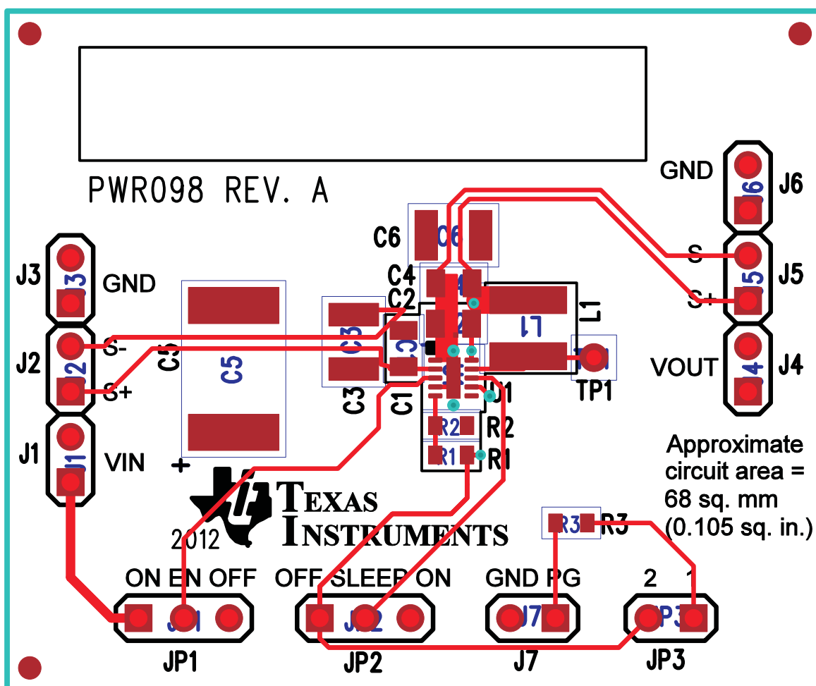
Figure 3. Assembly Layer
