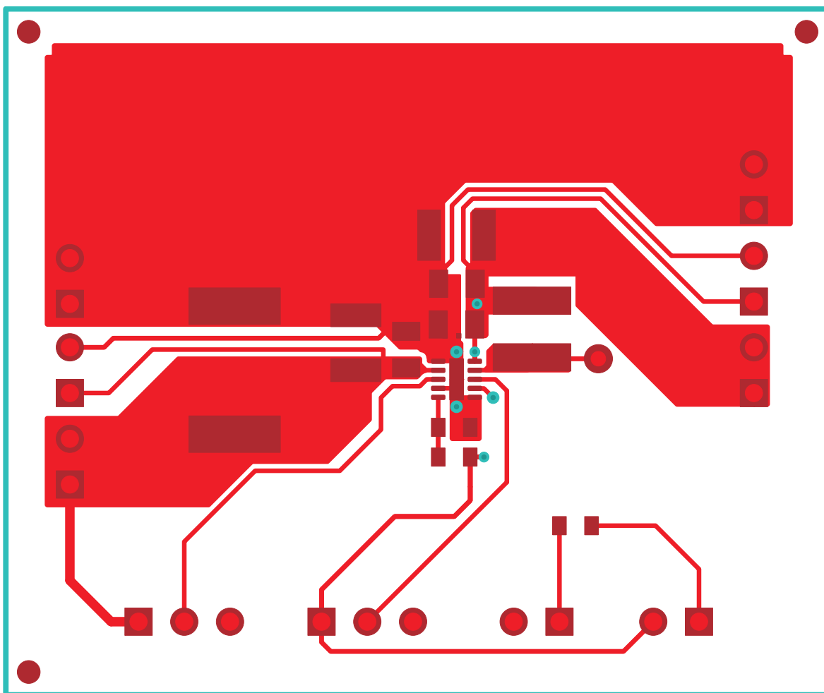
Figure 5. Top Layer
