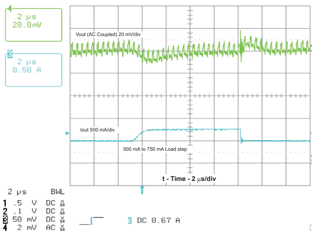
Figure 8. Load Transient Response With V_{in} = 12\text{ V}
