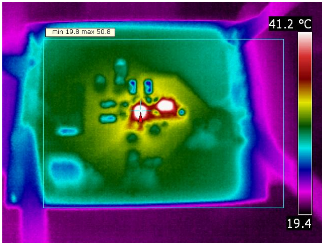
Figure 13. Thermal Performance With V_{in} = 12\text{ V} and I_{out} = 1\text{ A}
