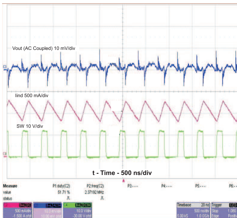
Figure 7. Output Voltage Ripple With V_{in} = 12\text{ V} and I_{out} = 1\text{ A}
