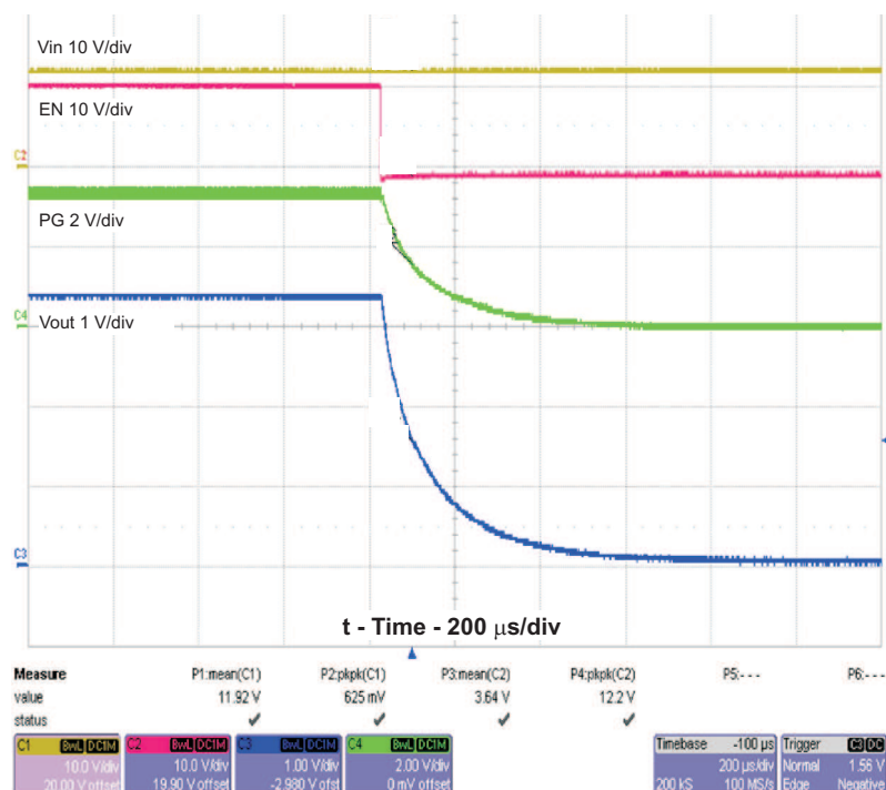
Figure 11. Shutdown on EN With 0.5-A Load
