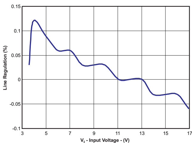
Figure 4. Line Regulation With I_{out} = 0.5 A
