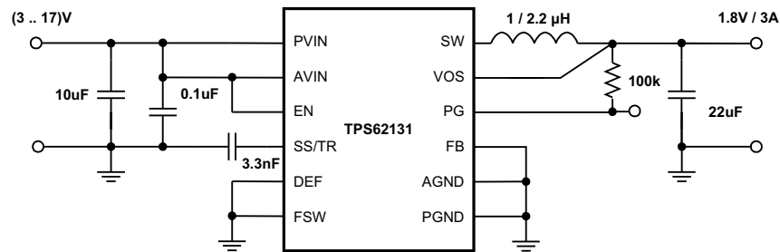
Figure 52. 1.8V/3A Power Supply
