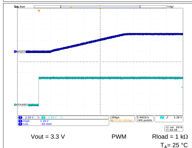
Figure 54. Start-Up Timing
