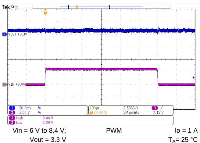
Figure 53. Line Transient Response
