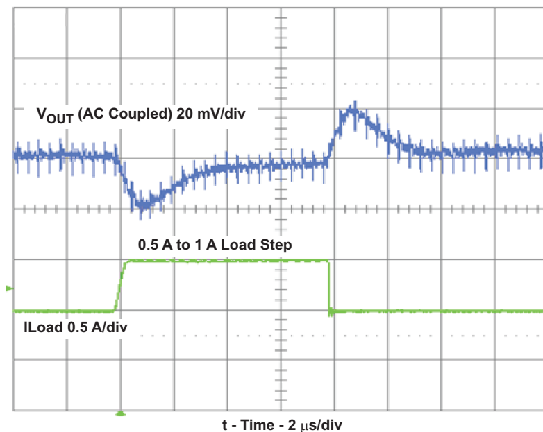
Figure 12. Load Transient Response With 2.2-μH Inductor and V_{in} = 12\text{ V}
