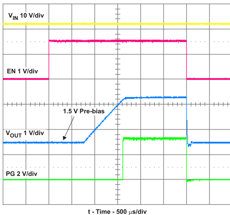
Figure 16. TPS62130A Prebias Start-Up and Shutdown on EN With 1-A Load and V_{\text{in}} = 12 \text{ V}
