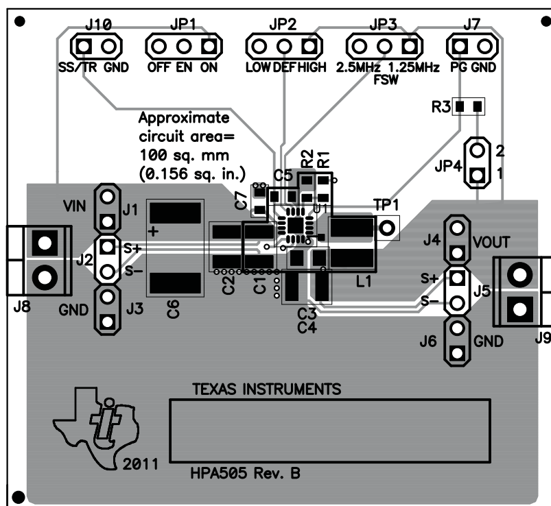
Figure 19. Assembly Layer
