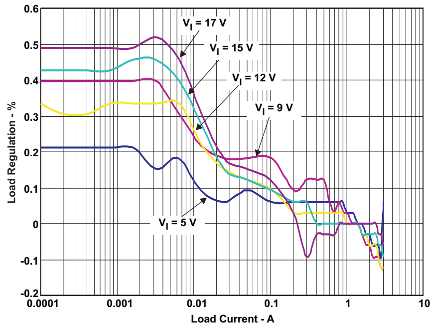
Figure 5. Load Regulation With 2.2-μH Inductor and FSW = LOW (high frequency)
