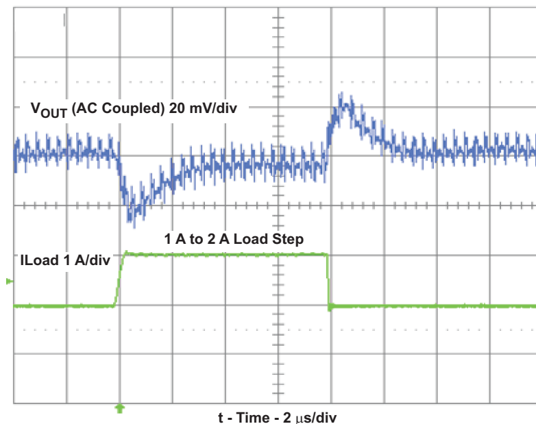
Figure 11. Load Transient Response With 1-μH Inductor and V_{in} = 12\text{ V}
