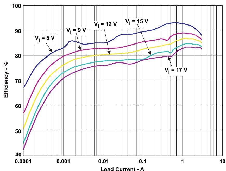
Figure 2. Efficiency With 1-μH Inductor and FSW = LOW (high frequency)
