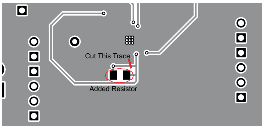
Figure 1. Loop Response Measurement Modification
