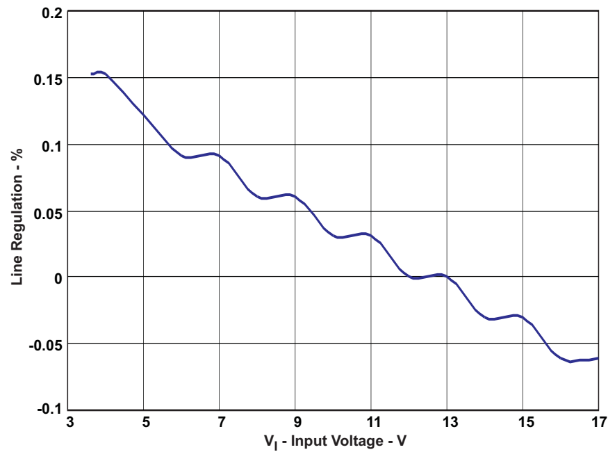
Figure 6. Line Regulation With 2.2-μH Inductor and FSW = LOW (high frequency) and I_{out} = 1\text{ A}
