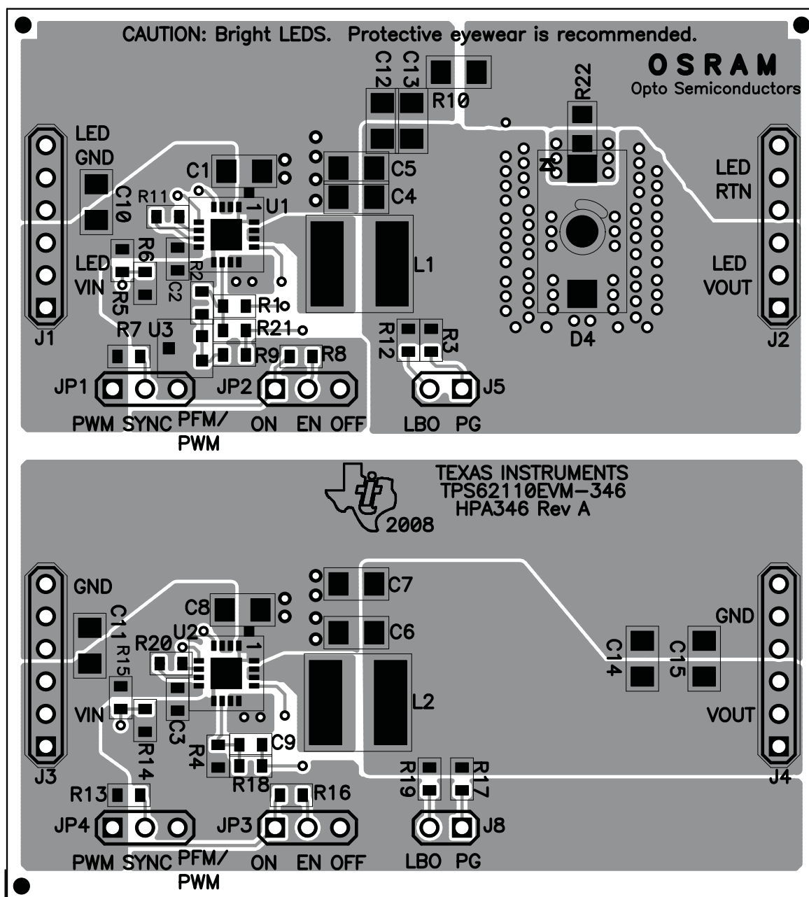
Figure 4. Assembly Layer
