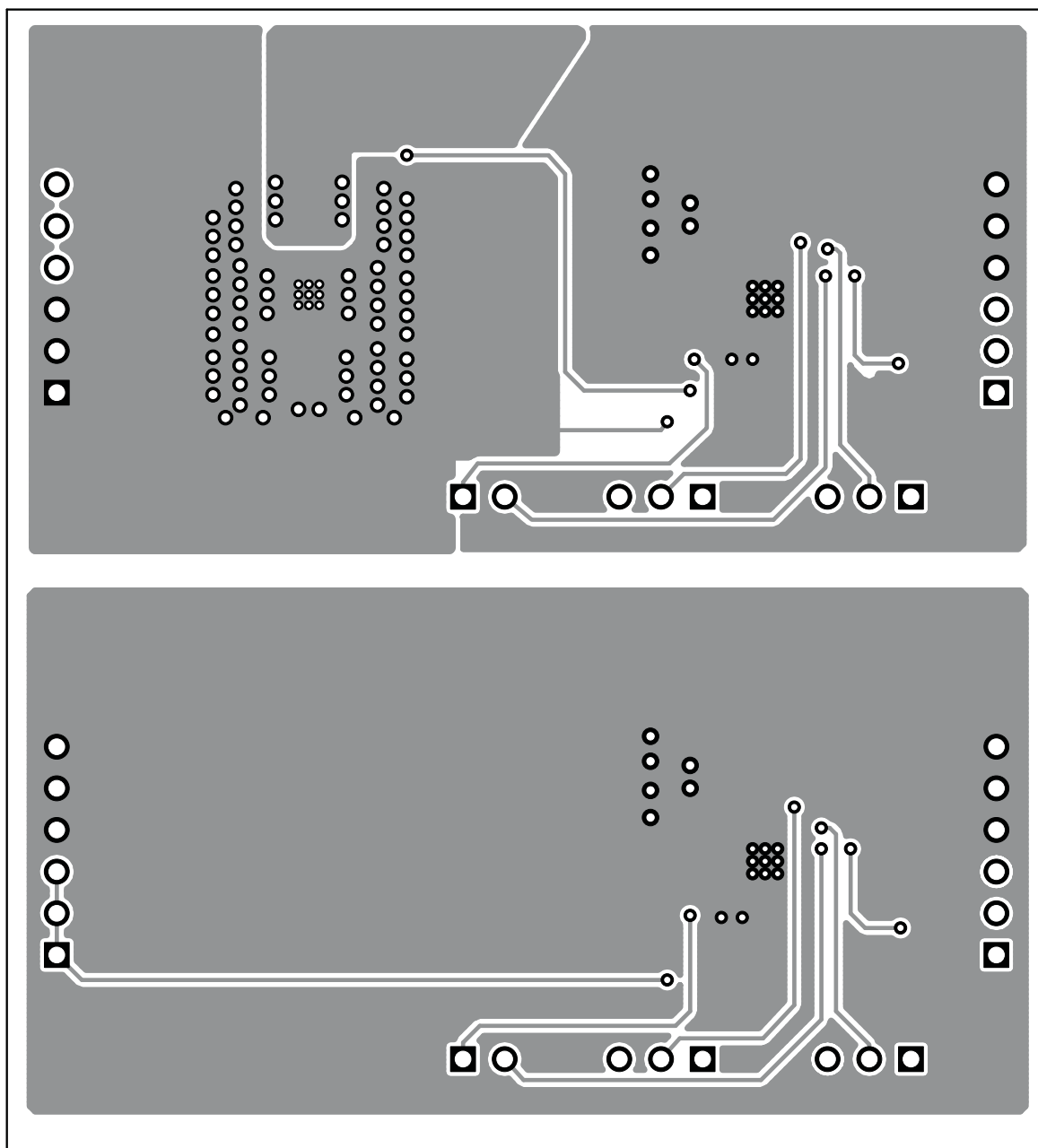
Figure 6. Bottom Layer Routing
